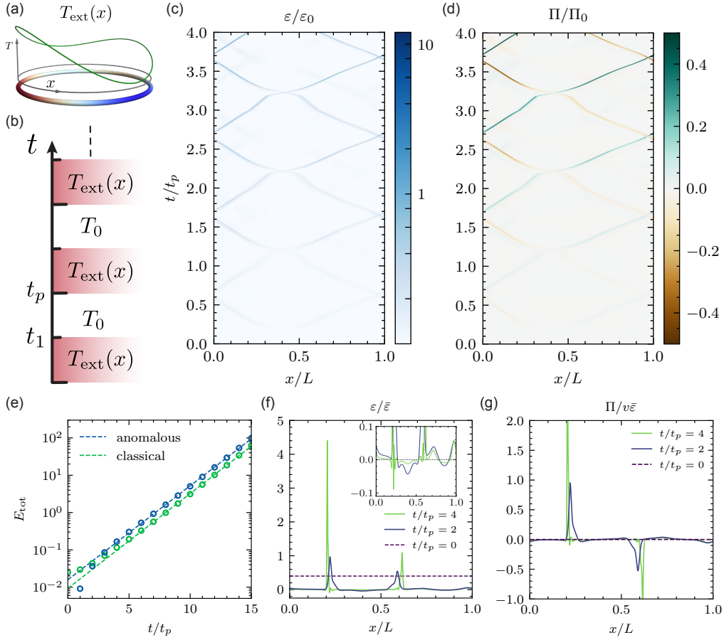
Figure 6: Floquet heating state . (a) We consider a ring of free relativistic fermions of velocity v_F = 1 . (b) This ring is driven periodically by an external temperature with a period t_p = t_1 + t_2 , such that (i) during time t_1 the external temperature is a smooth profile T_{\text{ext}}(x) varying around an average T_0 , shown in (a), and (ii) during time t_2 temperature is kept to a constant T_0 . The two times Lt_1/v_F = 0.1 and Lt_2/v_F = 0.45 , are chosen such that the period coincides with the time of flight of particles around the ring: L = v_F t_1 + \tilde{v}_F t_2 where \tilde{v}_F is the averaged effective velocity under the temperature profile T_{\text{ext}}(x) . (c) and (d) As a function of time, both the energy density \varepsilon and the momentum \Pi become highly inhomogeneous, and concentrate on a few trajectories. They are represented rescaled by the classical values \varepsilon_0 = v_F \Pi_0 = \gamma T_0^2 . The energy and momentum profiles are represented after two and four periods in panels (f) and (g), illustrating the localization mechanism. (e) Besides being focused spatially, the net energy of the ring E_{\text{tot}} = \int_0^L \varepsilon dx = L\bar{\varepsilon} increases: the Floquet state is heating. This is represented by monitoring the stroboscopic dynamics at times t_n = nt_p of the ring for which E_{\text{tot}} increases exponentially. Remarkably the rate of increase of this energy is not classical: quantum fluctuations, responsible for the trace and gravitational anomaly corrections, have a growing energy. The two focusing trajectories behave as heating black holes: in their neighborhood the energy density becomes negative, as shown in the inset of panel (f). This is an additional manifestation of the effects of quantum fluctuations induced by a local large curvature similar to those in a black-hole atmosphere.
