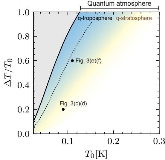
Figure 4: Diagram of the possible out of equilibrium thermodynamic states imposed by a temperature jump. The phase diagram corresponds to an imposed temperature profile, as represented in Fig. 3(b), varying between two temperatures T_{R/L} = T_0 \pm \Delta T/2 over a length \delta = 10 \mu\text{m} . The white region corresponds to the region with classical fluctuations where gravitational anomalies can be neglected. As in Fig. 2, the colored region signals the quantum atmosphere, and the color encodes the smooth crossover between the quantum stratosphere, where \varepsilon_q = \varepsilon_q^{(1)} \approx \varepsilon_q^{(2)} , and the quantum troposphere, where \varepsilon_q^{(1)} \neq \varepsilon_q^{(2)} . The relevance of quantum fluctuations is signaled by the relation \lambda_T(x) \gtrsim l_T(x) close to the temperature jump, between the thermal length \lambda_T and l_T = |\partial_x^2 T/T|^{-\frac{1}{2}} which characterises the temperature variation. The quantum troposphere is characterized by an additional length scale l_T^{(2)} = |\partial_x T/T|^{-1} \neq l_T defined by the imposed temperature profile. As in Fig. 2(a) the dotted line represents the state possessing black hole like thermodynamic local properties ( \varepsilon < 0 but T_{eq}^2 > 0 ). The thermodynamically forbidden region, in which the \varepsilon + P and the entropy are negative and our extended Luttinger correspondence does not apply, is shaded in gray. The two black dots represent the parameters chosen for Fig. 3. We chose the Fermi velocity to be v_F = 10^6 \text{m} \cdot \text{s}^{-1} , typical for relativistic materials.
