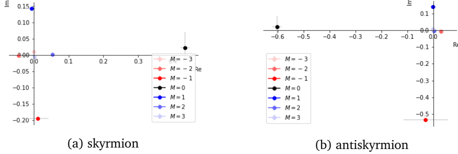
Figure 5: Plotting the numerically extracted multipole sources C_M seen in the general solution of the linearised Euler-Lagrange equations for solitons in a tilted field, \tilde{\psi}_{\text{lin}} = \sum_{M=-\infty}^{\infty} C_M e^{iM\phi} K_M(mr) , where the inverse decay lengthscale m = \sqrt{h_z - k^2 \sin^2 \theta_h} for DMI strength k , Zeeman interaction strength h_z .
