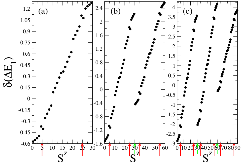
Figure 11: Differences of the first-order degenerate perturbation theory corrections of the energy \delta(\Delta E_1) = \Delta E_1(S^z + 1) - \Delta E_1(S^z) between successive S^z sectors of C_{60} away from the dimer limit \phi = \frac{\pi}{2} at the antiferromagnetic isotropic Heisenberg limit \omega = \frac{\pi}{4} of Hamiltonian (1) for \hbar = 0 and (a) s = \frac{1}{2} ( \Delta E_1 given in Table 10), (b) s = 1 ( \Delta E_1 given in Table 11), and (c) s = \frac{3}{2} ( \Delta E_1 given in Table 12). The (red) solid arrows show the locations of the \Delta S^z = 2 magnetization discontinuities, and the (green) long-dashed arrows the locations of standard \Delta S^z = 1 discontinuities which are due to the unperturbed energies (App. A).
