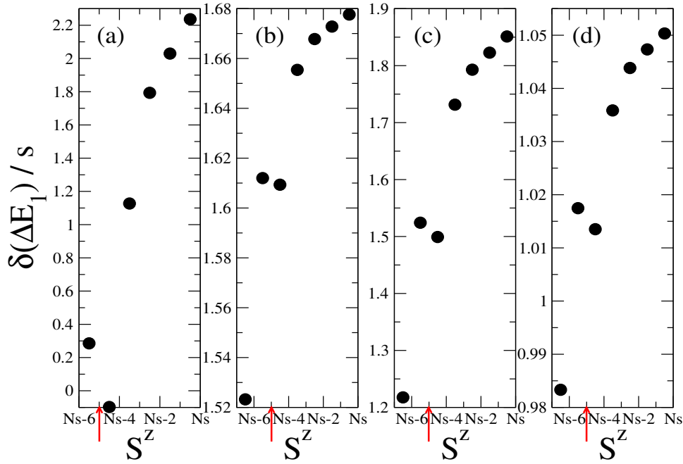
Figure 4: Differences of the first-order degenerate perturbation theory corrections of the energy over the spin magnitude \frac{\delta(\Delta E_1)}{s} = \frac{\Delta E_1(S^z+1)}{s} - \frac{\Delta E_1(S^z)}{s} between successive S^z sectors close to saturation for arbitrary s for (a) C_{20} (Table 4) and (b), (c), and (d) for C_{60} for \phi = \frac{\pi}{50} , \frac{\pi}{4} , and \frac{49}{100}\pi respectively (Table 6) away from the Ising limit \omega = 0 of Hamiltonian (1) for h = 0 . The (red) solid arrows show the locations of the \Delta S^z = 2 magnetization discontinuities.
