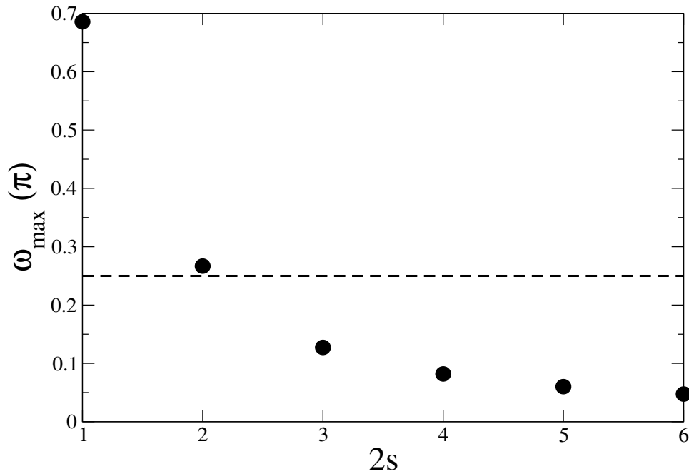
Figure 7: Maximum value \omega_{max} as a function of s for which the ground state of Hamiltonian (1) for C_{20} has a \Delta S^z = 2 magnetization discontinuity five spin flips away from saturation. The dashed line shows the isotropic Heisenberg limit \omega = \frac{\pi}{4} .
