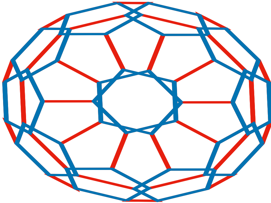
Figure 8: Truncated icosahedron C_{60} . The blue lines correspond to the twelve pentagons and the intrapentagon bonds and their exchange interaction strength J_1 \equiv \cos\phi , while the red lines to the interpentagon (dimer) bonds and their exchange interaction strength J_2 \equiv \sin\phi .
