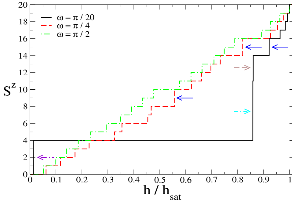
Figure 6: S^z as a function of the magnetic field h over the saturation field h_{sat} in the ground state of Hamiltonian (1) for C_{20} for s = 1 . The (black) solid line corresponds to \omega = \frac{\pi}{20} , the (red) long-dashed line to \omega = \frac{\pi}{4} , and the (green) long-dashed-dotted line to \omega = \frac{\pi}{2} . The (blue) solid arrows point to the discontinuities with \Delta S^z = 2 , the (brown) long-dashed arrow to the discontinuity with \Delta S^z = 3 , the (violet) long-dashed-dotted arrow to the discontinuity with \Delta S^z = 4 , and the (cyan) double-dashed-dotted arrow to the discontinuity with \Delta S^z = 7 .
