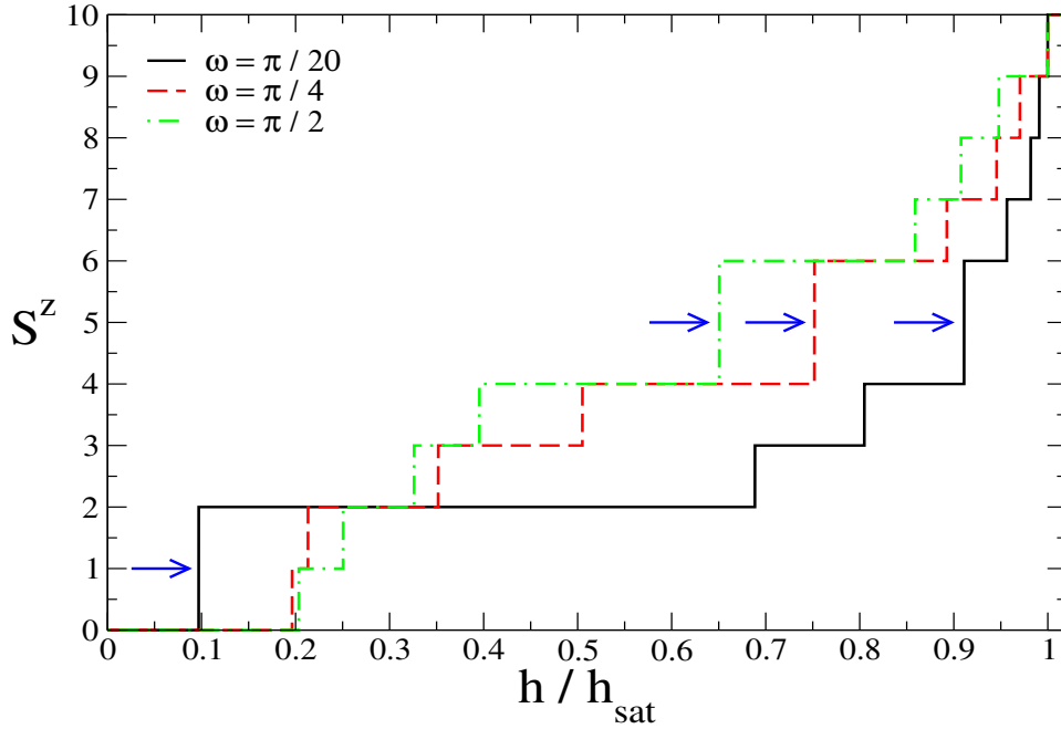
Figure 5: S^z as a function of the magnetic field h over the saturation field h_{sat} in the ground state of Hamiltonian (1) for C_{20} for s = \frac{1}{2} . The (black) solid line corresponds to \omega = \frac{\pi}{20} , the (red) long-dashed line to \omega = \frac{\pi}{4} , and the (green) long-dashed-dotted line to \omega = \frac{\pi}{2} . The (blue) solid arrows point to the discontinuities with \Delta S^z = 2 .
