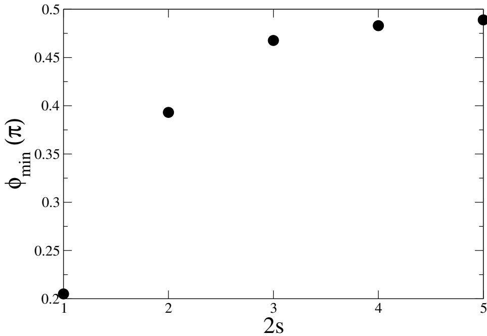
Figure 10: Minimum value \phi_{min} as a function of s for which the ground state of Hamiltonian (1) for C_{60} has a \Delta S^z = 2 magnetization discontinuity five spin flips away from saturation at the isotropic Heisenberg limit \omega = \frac{\pi}{4} .
