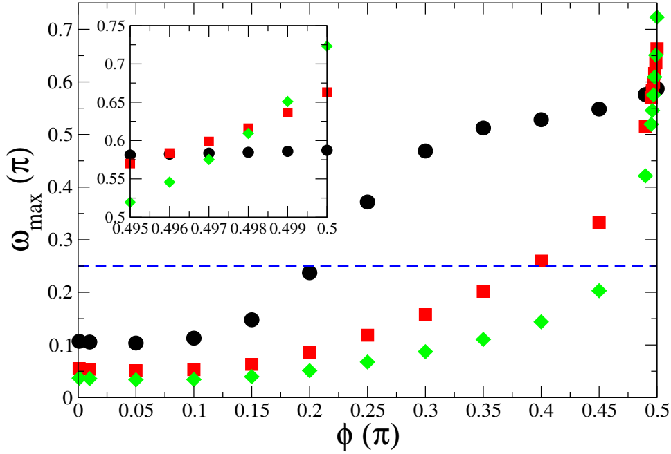
Figure 9: Maximum value \omega_{max} for which the s = \frac{1}{2} (black circles), 1 (red squares), and \frac{3}{2} (green diamonds) ground state of Hamiltonian (1) for C_{60} has a \Delta S^z = 2 magnetization discontinuity between S^z = Ns - 6 and Ns - 4 as a function of \phi = \tan^{-1} \frac{J_2}{J_1} , which determines the relative strength of the two symmetrically independent exchange interactions. The dashed line shows the isotropic Heisenberg limit \omega = \frac{\pi}{4} . The inset focuses on the high range of \phi .
