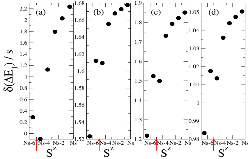
Figure 4: Differences of the first-order degenerate perturbation theory corrections of the energy over the spin magnitude \frac{\delta(\Delta E_1)}{s} = \frac{\Delta E_1(S^z+1)}{s} - \frac{\Delta E_1(S^z)}{s} between successive S^z sectors close to saturation for arbitrary s for (a) C_{20} (Table 4) and (b), (c), and (d) for C_{60} for \phi = \frac{\pi}{50} , \frac{\pi}{4} , and \frac{49}{100}\pi respectively (Table 6) away from the Ising limit \omega = 0 of Hamiltonian (1) for h = 0 . The (red) solid arrows show the locations of the \Delta S^z = 2 magnetization discontinuities.
