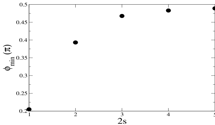
Figure 10: Minimum value \phi_{min} as a function of s for which the ground state of Hamiltonian (1) for C_{60} has a \Delta S^z = 2 magnetization discontinuity five spin flips away from saturation at the isotropic Heisenberg limit \omega = \frac{\pi}{4} .
