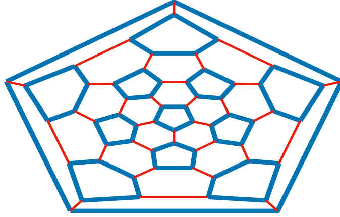
Figure 8: Planar projection of the truncated icosahedron C_{60} . The (blue) thick lines correspond to the twelve pentagons and the intrapentagon bonds and their exchange interaction strength J_1 \equiv \cos\phi , while the (red) thin lines to the interpentagon (dimer) bonds and their exchange interaction strength J_2 \equiv \sin\phi .
