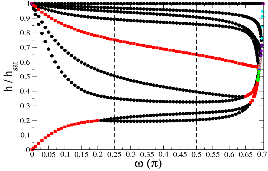
Figure 2: Magnetic fields h over the saturation field h_{sat} for which ground-state magnetization discontinuities occur as a function of \omega in the ground state of Hamiltonian (1) for C_{20} for s = \frac{1}{2} . The (black) circles correspond to discontinuities with \Delta S^z = 1 , the (red) squares with \Delta S^z = 2 , the (green) diamonds with \Delta S^z = 3 , the (blue) triangles up with \Delta S^z = 6 , the (brown) triangles left with \Delta S^z = 7 , the (violet) triangles down with \Delta S^z = 8 , the (cyan) triangles right with \Delta S^z = 9 , and the (magenta) \times 's with \Delta S^z = 10 . The (black) dashed lines show the isotropic Heisenberg ( \omega = \frac{\pi}{4} ) and the XX ( \omega = \frac{\pi}{2} ) limit.
