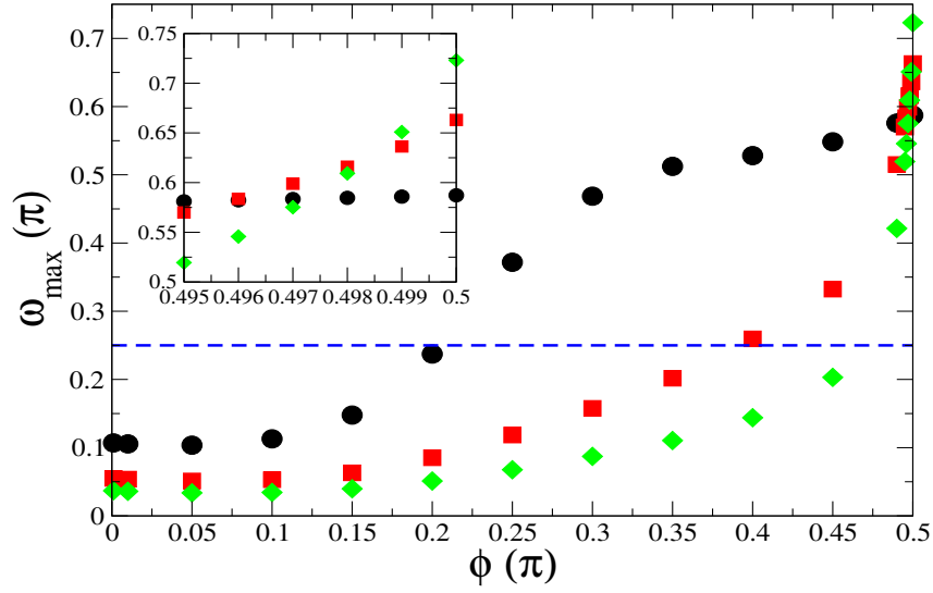
Figure 9: Maximum value \omega_{max} for which the s = \frac{1}{2} (black circles), 1 (red squares), and \frac{3}{2} (green diamonds) ground state of Hamiltonian (1) for C_{60} has a \Delta S^z = 2 magnetization discontinuity between S^z = Ns - 6 and Ns - 4 as a function of \phi = \tan^{-1} \frac{J_2}{J_1} , which determines the relative strength of the two symmetrically independent exchange interactions. The dashed line shows the isotropic Heisenberg limit \omega = \frac{\pi}{4} . The inset focuses on the high range of \phi .
