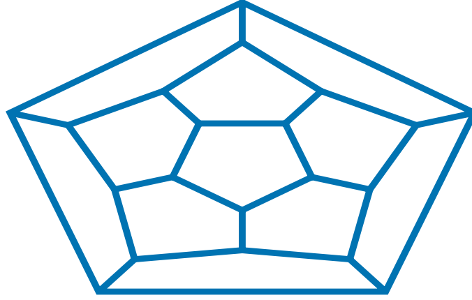
Figure 1: Planar projection of the dodecahedron C_{20} .
