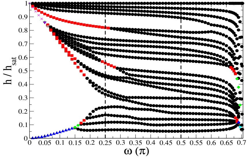
Figure 3: Magnetic fields h over the saturation field h_{sat} for which ground-state magnetization discontinuities occur as a function of \omega in the ground state of Hamiltonian (1) for C_{20} for s = 1 . The (black) circles correspond to discontinuities with \Delta S^z = 1 , the (red) squares with \Delta S^z = 2 , the (green) diamonds with \Delta S^z = 3 , the (blue) triangles up with \Delta S^z = 4 , the (brown) triangles left with \Delta S^z = 6 , the (violet) triangles down with \Delta S^z = 7 , the (cyan) triangles right with \Delta S^z = 9 , the (magenta) \times 's with \Delta S^z = 10 , and the (indigo) stars with \Delta S^z = 16 . The (black) dashed lines show the isotropic Heisenberg ( \omega = \frac{\pi}{4} ) and the XX ( \omega = \frac{\pi}{2} ) limit.
