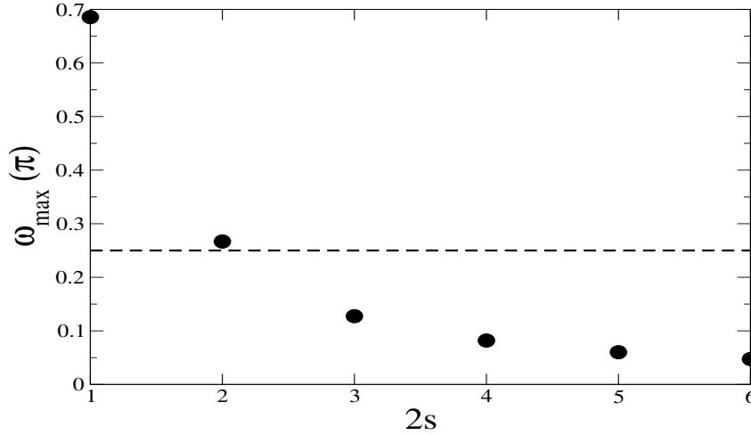
Figure 7: Maximum value \omega_{max} as a function of s for which the ground state of Hamiltonian (1) for C_{20} has a \Delta S^z = 2 magnetization discontinuity five spin flips away from saturation. The dashed line shows the isotropic Heisenberg limit \omega = \frac{\pi}{4} .
