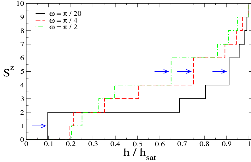
Figure 5: S^z as a function of the magnetic field h over the saturation field h_{sat} in the ground state of Hamiltonian (1) for C_{20} for s = \frac{1}{2} . The (black) solid line corresponds to \omega = \frac{\pi}{20} , the (red) long-dashed line to \omega = \frac{\pi}{4} , and the (green) long-dashed-dotted line to \omega = \frac{\pi}{2} . The (blue) solid arrows point to the discontinuities with \Delta S^z = 2 .
