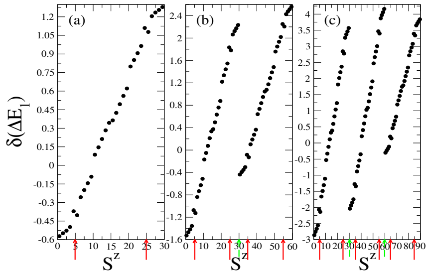
Figure 11: Differences of the first-order degenerate perturbation theory corrections of the energy \delta(\Delta E_1) = \Delta E_1(S^z + 1) - \Delta E_1(S^z) between successive S^z sectors of C_{60} away from the dimer limit \phi = \frac{\pi}{2} at the antiferromagnetic isotropic Heisenberg limit \omega = \frac{\pi}{4} of Hamiltonian (1) for h = 0 and (a) s = \frac{1}{2} ( \Delta E_1 given in Table 10), (b) s = 1 ( \Delta E_1 given in Table 11), and (c) s = \frac{3}{2} ( \Delta E_1 given in Table 12). The (red) solid arrows show the locations of the \Delta S^z = 2 magnetization discontinuities, and the (green) long-dashed arrows the locations of standard \Delta S^z = 1 discontinuities which are due to the unperturbed energies (App. A).
