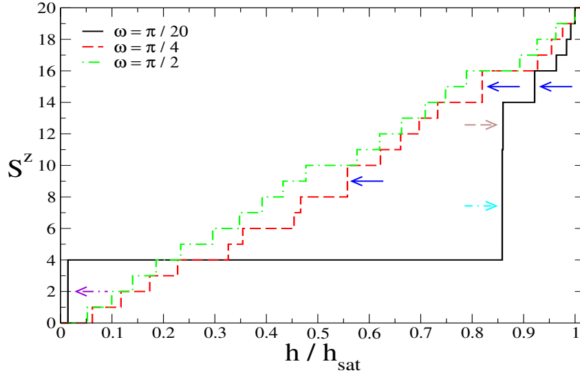
Figure 6: S^z as a function of the magnetic field h over the saturation field h_{sat} in the ground state of Hamiltonian (1) for C_{20} for s = 1 . The (black) solid line corresponds to \omega = \frac{\pi}{20} , the (red) long-dashed line to \omega = \frac{\pi}{4} , and the (green) long-dashed-dotted line to \omega = \frac{\pi}{2} . The (blue) solid arrows point to the discontinuities with \Delta S^z = 2 , the (brown) long-dashed arrow to the discontinuity with \Delta S^z = 3 , the (violet) long-dashed-dotted arrow to the discontinuity with \Delta S^z = 4 , and the (cyan) double-dashed-dotted arrow to the discontinuity with \Delta S^z = 7 .
