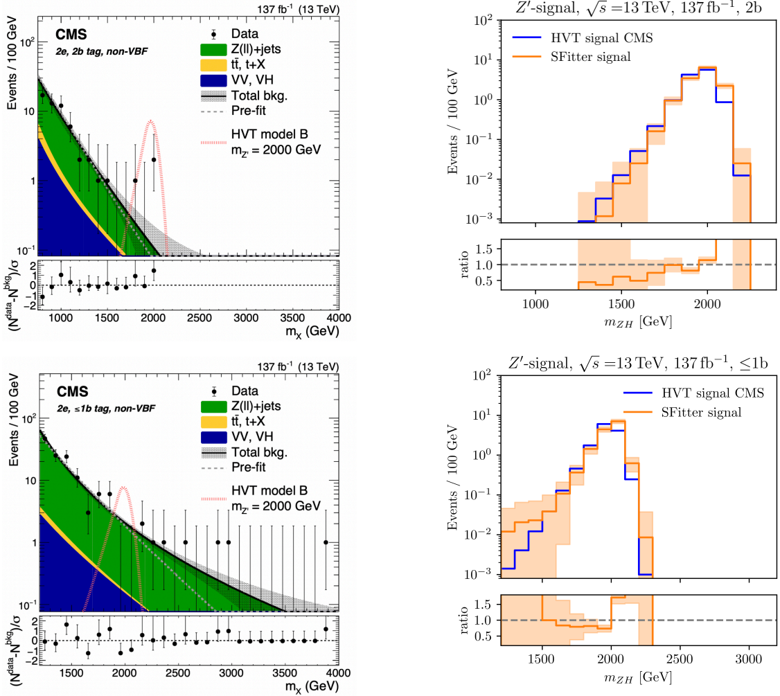
Figure 15: Left: measured m_{ZH} distributions for the two b -tagging categories [79]. Right: comparison between the Z' signal quoted by CMS and our estimate. The orange bands show the statistical uncertainty from the Monte Carlo generation.
