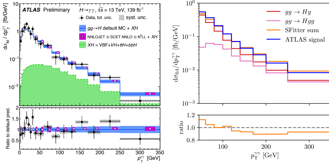
Figure 17: Left: measured d\sigma_{\text{fid}}/dp_T^{\gamma\gamma} distribution [80]. Right: comparison between the the ATLAS distribution and our SM estimate summing contributions from gg \rightarrow Hg and gg \rightarrow Hgg .
