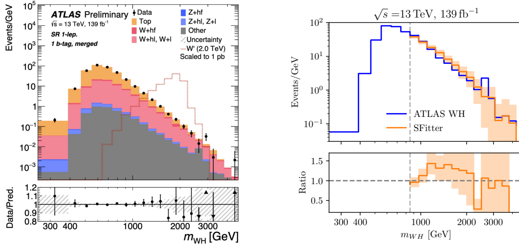
Figure 12: Left: measured m_{WH} distribution [78]. Right: comparison between the the ATLAS results and our SM background estimate. The orange band shows the statistical uncertainty from the Monte Carlo generation.
