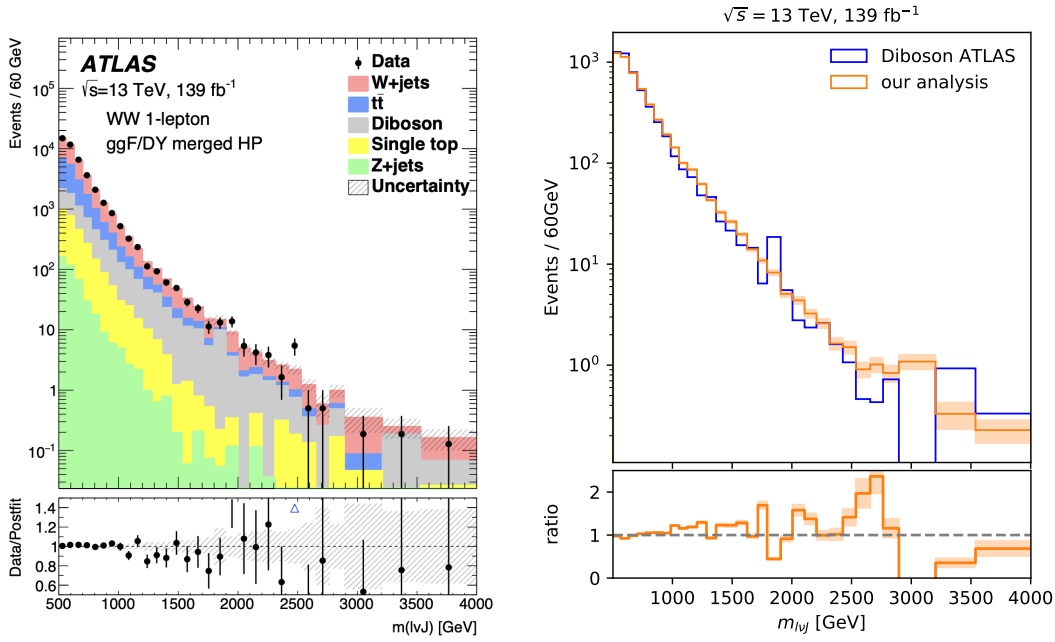
Figure 10: Left: measured m_{VV} distribution [71]. Right: comparison between ATLAS results and our SM background estimate. The orange band shows the statistical uncertainty from the Monte Carlo generation.
