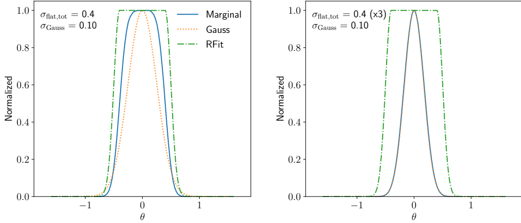
Figure 1: Marginalized and profiled likelihoods from the convolution of a Gaussian distribution with one (left) and three (right) flat ones. The orange curve shows, for comparison, the Gaussian obtained adding half-widths in quadrature.
