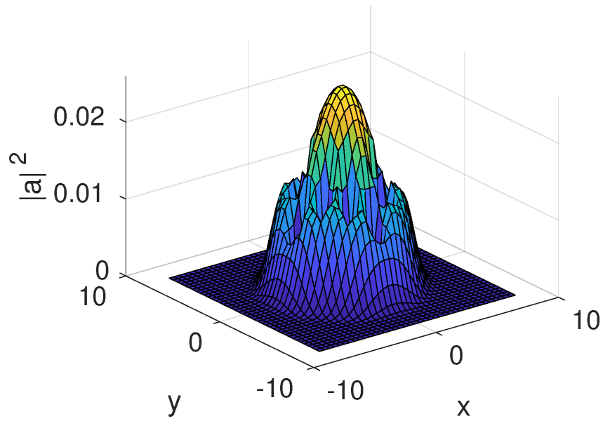
GPEvortex2D #1 , t = 15.000
