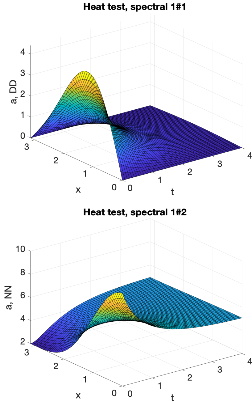
Figure 23: Top figure: Spectral solution for a as a function of time and position with Dirichlet-Dirichlet boundaries. Bottom figure: Plot of the solution with Neumann-Neumann boundaries.
