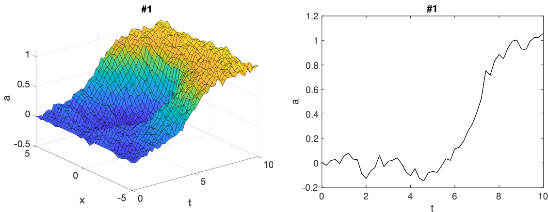
Figure 8: Two space-dimensional example graphs, direct differentiation.
