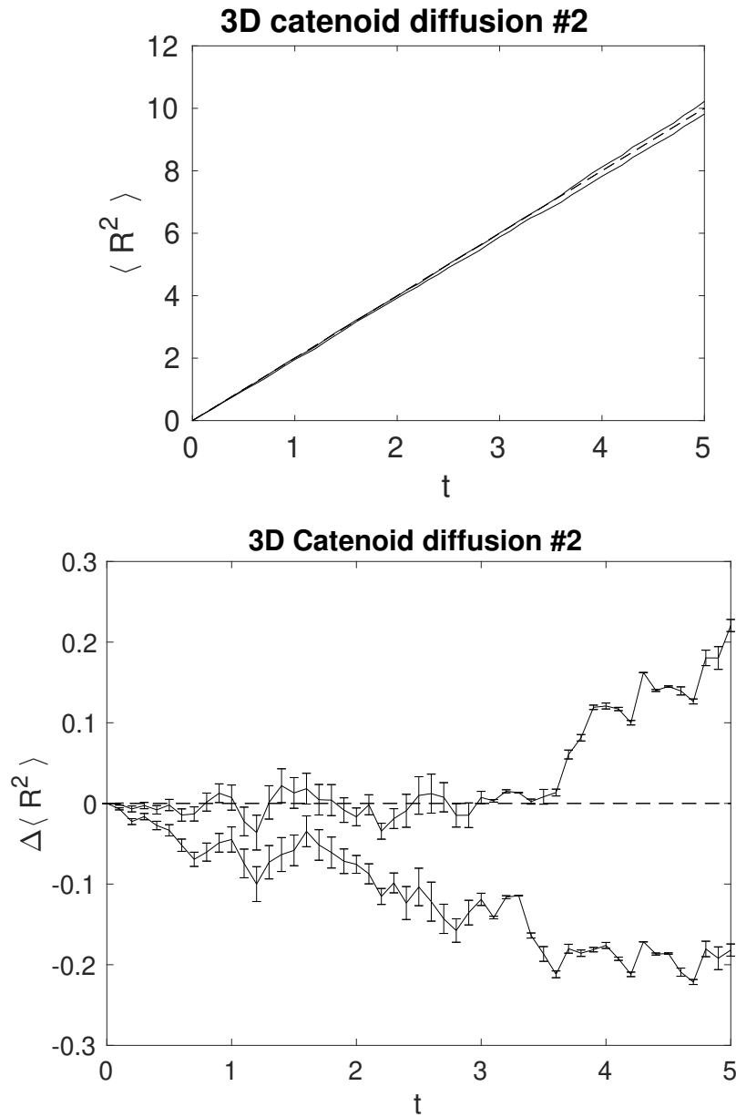
Figure 24: Top figure: Computed time evolution of the catenoid squared Euclidean diffusion distance |\mathbf{x}_0 - \mathbf{x}(t)|^2 , where \mathbf{x}_0 = (1, 0, 0)^T , as a function of time. Bottom figure: Differences between the computed time evolution of the catenoid squared Euclidean distance |\mathbf{x}_0 - \mathbf{x}(t)|^2 and the exact result. In both cases the solid lines indicate the stochastic error bounds, error-bars are the time-step errors, while the dashed line indicates the theoretical prediction.
