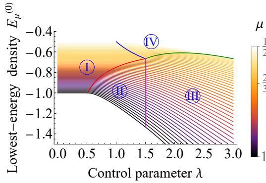
Figure 2: Lowest-energy density E_{\mu}^{(0)}(\epsilon, \lambda) of the parental case (7) for different values of the control parameter \lambda and the unirep continuous parameter \mu , varying from \mu = 1 (black curve) to \mu = 1/2 (light yellow curve), with a step size of \delta\mu = 0.01 . There are four different quantum phases in the phase diagram, which coincide at a quadruple point (\lambda, \mu)_q = (3/2, 2/3) . The phases are separated by curves of critical points in color red, magenta, green, and blue. Both axes are in \epsilon units.
