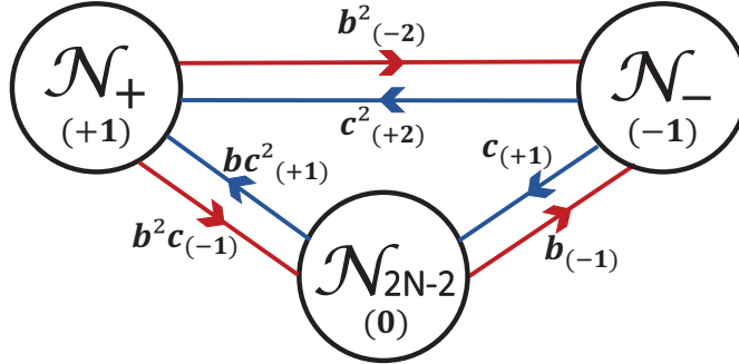
Figure 15: The topological quiver representing \mathcal{L}_{so_{2N}}^{vect} . It has three nodes and 6 links. The nodes describe self-dual topological matter and the links describe topological bi-matter.
