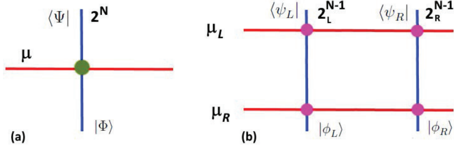
Figure 18: On the left, a horizontal spinorial like 't Hooft line crossing a vertical Wilson line carrying internal fermionic states \Psi = (\psi_L, \psi_R) . On the right, the structure of the coupling under the Levi decomposition showing chiral and antichiral Weyl states traveling along vertical lines.
