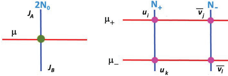
Figure 19: On the left, a horizontal spinorial like 't Hooft line crossing a vertical Wilson line carrying a bosonic current J^A = \Psi \Gamma^A \Psi . On the right, The splitting of the current into two currents u_i = \Psi \Upsilon_i \Phi and \bar{v}^i = \Psi \bar{\Upsilon}^i \Phi traveling along the vertical lines.
