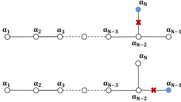
Figure 17: Dynkin diagram of D_N Lie algebras where the two Levi decompositions with respect to the spinorial coweights are illustrated by : (a) removing the simple root \alpha_N for the minuscule coweight \mu_N . (b) removing the simple root \alpha_{N-1} for the minuscule coweight \mu_{N-1} .
