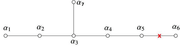
Figure 25: Dynkin Diagram of E_7 having seven nodes labeled by the simple roots \alpha_i . The cross ( \times ) indicates the root cut by the Levi decomposition where the Levi subgroup is SO_2 \times E_6 .
