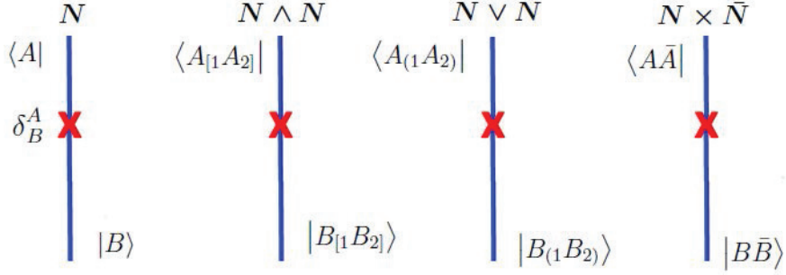
Figure 2: Four examples of Wilson lines in different representations of sl_N occupying vertical lines in \mathbb{R}^2 ( x=cte ); they carry different electric charges. The representation \mathbf{R} and the type of incoming quantum states are indicated above each line, while the outgoing states are given at the bottom of the line. The red cross indicates a local interaction point.
