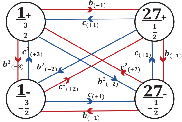
Figure 28: The topological quiver Q_{E_7} representing \mathcal{L}_{E_7} . It has 4 nodes and 12 links. The nodes describe self-dual topological matter. The links describe bi-matter in (R_i, \bar{R}_j) of E_6 charged under SO(2) with charges \pm 1, \pm 2, \pm 3 .
