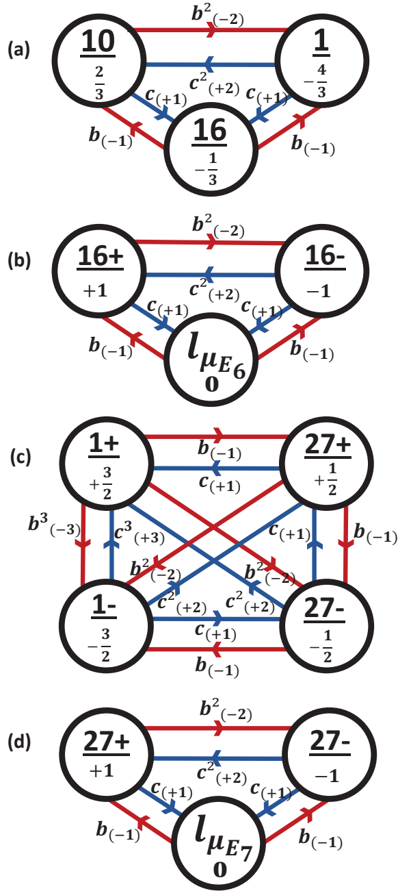
Figure 31: Leading elements of topological quiver digrams for the L-operators of E- type. The first two quivers for the E_6 gauge theory. (a) for the fundamental 27 of E_6 ; and (b) for the adjoint representation. The last two quivers regard the E_7 Chern-Simons theory. (c) for the fundamental 56 of E_7 and (d) for the adjoint representation.
