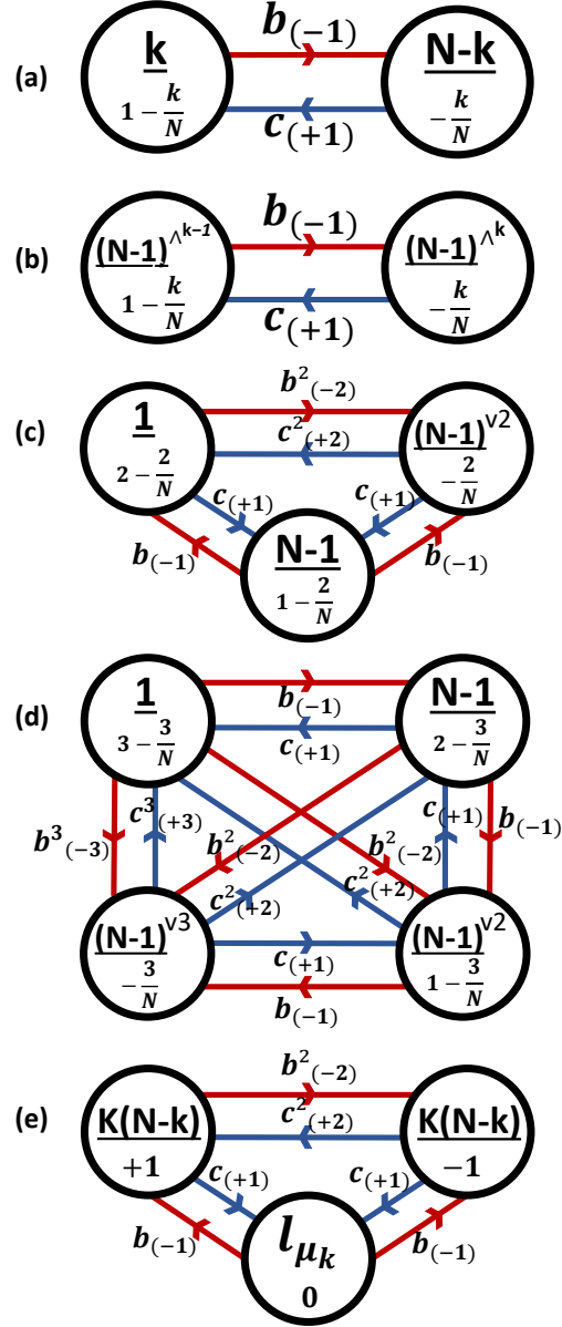
Figure 29: Leading elements of topological quiver digrams for the L-operators of A-type. These quivers are classified by the magnetic charge \mu_k of the 't Hooft line and the representation \mathbf{R} . (a) Wilson line with charge \mathbf{R} = N . (b) Wilson line with \mathbf{R} = N^k . (c) Wilson line with \mathbf{R} = N^2 . (d) Wilson line with \mathbf{R} = N^3 . (e) Wilson line with charge \mathbf{R} = \text{adj } sl_N .
