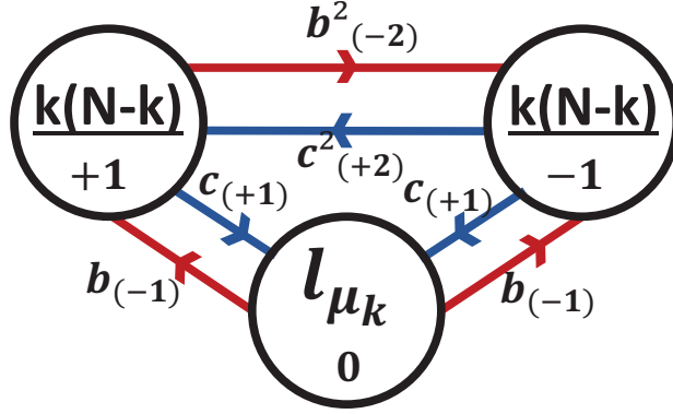
Figure 11: The topological quiver Q_{adj(sl_N)}^{\mu_k} for the adjoint representation of sl_N . It has three nodes \mathcal{N}_0 = l_{\mu_k} and \mathbf{n}_{\pm} = \mathbf{k}(N - \mathbf{k})_{\pm} .
