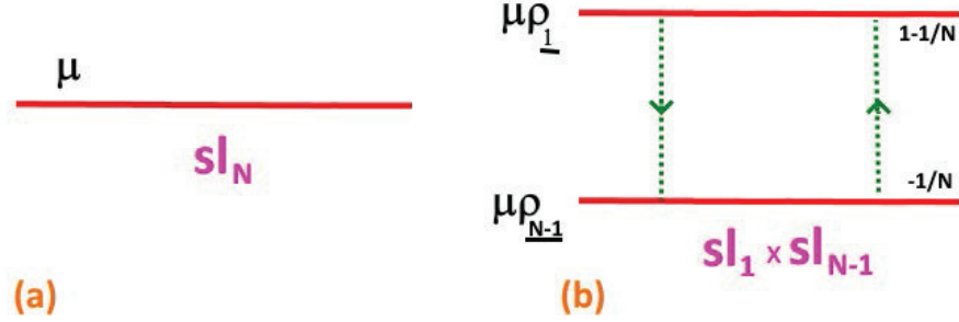
Figure 6: (a) Magnetic 'tHooft with charge \mu_1 from the point of view of global sl_N symmetry. (b) The same line from the point of view of internal sl_1 \oplus sl_{N-1} . here, the line \mu splits into two sublimes \mu\rho_1 and \mu\rho_{N-1} as described in eq(2.25).
