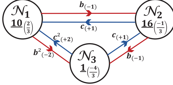
Figure 24: \mathcal{L}_{E_6} as a topological quiver with 3 nodes and 6 links. The nodes are given by the self-dual R_i \otimes \bar{R}_i and the links by bi-matter R_i \otimes \bar{R}_j . In addition to SO_{10} representations, the Darboux coordinates b^\alpha, c_\alpha carry SO_2 charges given by q = \pm 1 . The fundamental vector-like matter V^i and W_i carry -2 and +2 .
