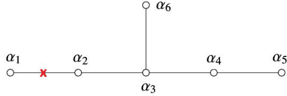
Figure 21: The Dynkin Diagram of e_6 having six nodes labeled by the simple roots \alpha_i . The cross ( \times ) indicates the cutted node in the Levi decomposition with respect to \mu_1 , the Levi subalgebra in this case is given by so(10) \oplus so(2) .
