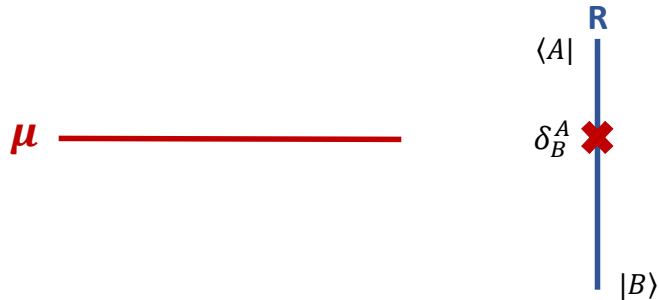
Figure 1: Line defects in the real plane \mathbb{R}^2 . On the left, a horizontal 't Hooft line with magnetic charge \mu expanding along the x-axis ( y = 0 ) at z = 0 . On the right, a vertical Wilson line expanding along the y-axis ( x = 0 ) at z \neq 0 with electric charge in some representation \mathbf{R} . Notice that the 't Hooft line is in fact paired to a similar one located at z = \infty with magnetic charge -\mu [52].
