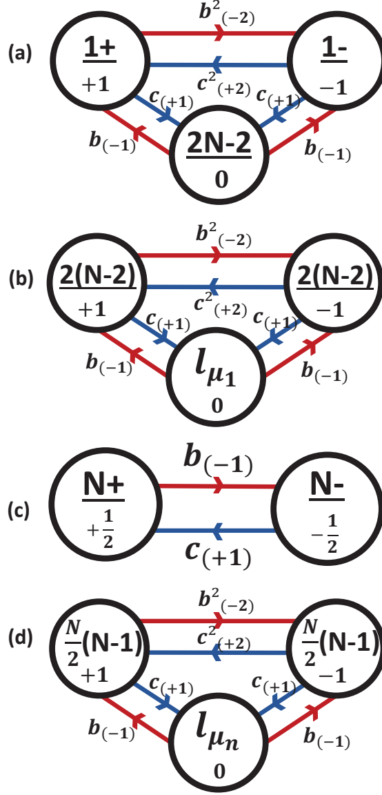
Figure 30: Leading elements of topological quiver digrams for the L-operators of D-type. The first two quivers correspond to the Levi decomposition with respect to the (vectorial) minuscule coweight \mu_1 : (a) Wilson line with charge \mathbf{R} = 2\mathbf{N} . (b) Wilson line with \mathbf{R} = \mathbf{adjso}_{2N} . The other two quivers correspond to the Levi decomposition with respect to the (spinorial) minuscule coweight \mu_N : (c) Wilson line with \mathbf{R} = 2^{N-1} . (d) Wilson line with \mathbf{R} = \mathbf{adjso}_{2N} .
