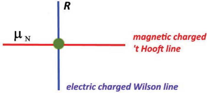
Figure 16: A horizontal 't Hooft line of D- type with spinor-like magnetic charge given by the minuscule coweight \mu_N of SO_{2N} couples to a vertical Wilson line characterized by a representation \mathbf{R} of so_{2N} .
