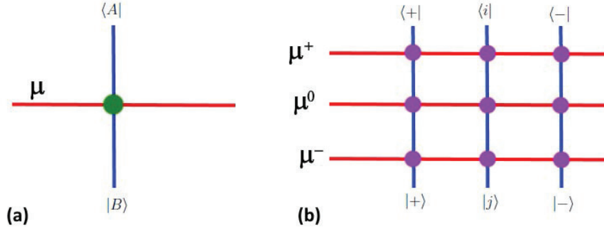
Figure 12: (a) A horizontal vector-like 't Hooft line with magnetic charge \mu_1 crossing an electrically charged vertical Wilson line. The green dot refers to the coupling between the two lines; it is given by the Lax operator \mathcal{L}_R^{\mu_1} . (b) Intrinsic structure of the Lax operator interpreted in terms of a topological gauge quiver with three nodes and 6 links.
