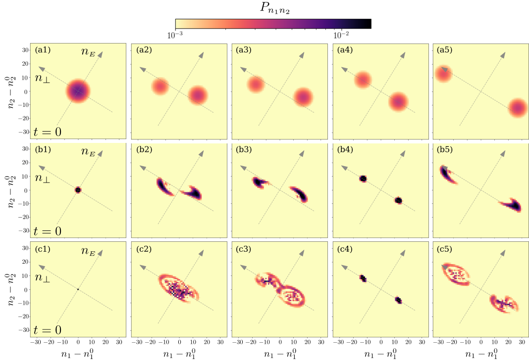
Figure 3: Typical dynamics of adiabatic cat states. Distribution of number of quanta of the two modes P_{n_1 n_2} = \langle n_1, n_2 | \hat{\rho}_{12} | n_1, n_2 \rangle at different times for three initial states. The modes are prepared in a Gaussian state with an average value of phase \phi_1^0 = \phi_2^0 = 0 and an equal width in number of quanta \Delta n_1 = \Delta n_2 = \Delta n , corresponding to a width \Delta\phi = 1/(2\Delta n) in phase. The qubit is prepared in (|\uparrow\rangle + |\downarrow\rangle)/\sqrt{2} . The evolution of states with different initial width \Delta n is represented: line (a), \Delta n = 5 , \Delta\phi \simeq 0.03\pi ; line (b), \Delta n = 0.7 , \Delta\phi \simeq 0.23\pi , and line (c), Quasi-Fock state \Delta n = 1/(2\pi) , delocalized in phase \Delta\phi = \pi . The columns (2) to (5) represent the time evolved state at respectively t = 8/3 , 16/3 , 8 and t = 32/3 in units of the period of the first mode T_1 = 2\pi/\omega_1 . The dynamics splits the initial state in a cat state in the sense of a superposition of two states with distinguishable energy content.
