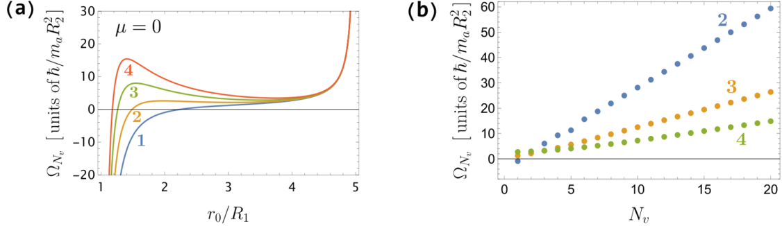
Figure 8: Uniform precession of a massless necklace for the same annular geometry as in Fig. 2. (a) Angular velocity as a function of the radius of the orbit for different numbers of vortices N_v (the numbers label the value of N_v for each curve). (b) Angular velocity as a function of the number of vortices for different radii of the orbit r_0/R_1 (the numbers refer to the value of r_0/R_1 for each curve).
