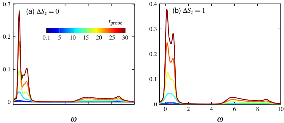
Figure 6: (a) Spin conserving and (b) non-conserving RIXS channels for a Mott insulating Hubbard chain with U = 8 , U_c = 1.5 , \Gamma = 0.1 , L = 64 sites, for different probing times t_{probe} . The inelastic features at low energies emerge after a characteristic time for the electrons to break and decay into spinons and doublons.
