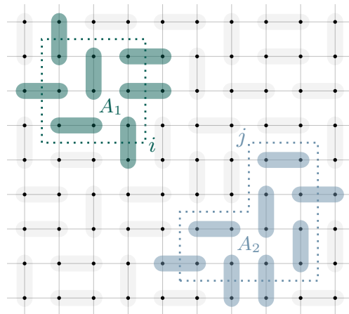
FIG. 1. Illustration of the tripartite geometry we consider for a specific configuration of the dimer model. In this example, the graph is the square lattice, and A_1 , A_2 , and B are tiled with green, blue, and gray dimers, respectively. The boundary dimers are those that cross the boundaries (dotted lines) of the subsystems. Indices i and j correspond to the boundary configurations between B and A_1 or A_2 , respectively.
