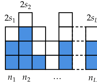
FIG. 1. The pole configurations of the elliptic genus give rise to a restricted occupancy problem. Each column with at most s_\alpha blue boxes corresponds to a spin- s_\alpha state at each site of the spin chain. The total number of blue boxes is M .
