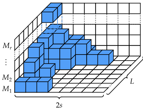
FIG. 3. A 3d restricted occupancy problem. On each level we have a 2d restricted occupancy with n_\alpha^{(a)} boxes in each row and a total of M_a boxes. Each row on a higher level has no more boxes than the lower level.
