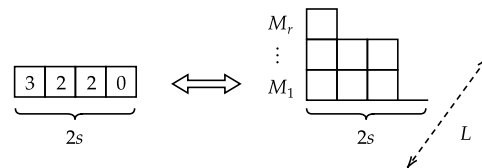
FIG. 4. At each site, the \mathfrak{su}(r+1) weight labelled by a semi-standard Young tableau corresponds to a partition in the 3d restricted occupancy problem.
