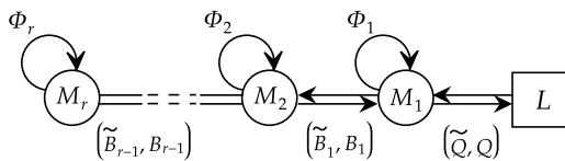
FIG. 2. The linear quiver gauge theory corresponding to the SU(r+1) spin chain.
