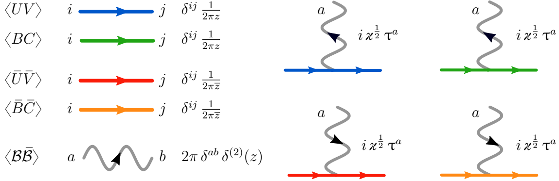
Figure 3: Feynman rules of the model (4.1). We have expanded \mathcal{B} = \sum \mathcal{B}_a \tau^a , where \mathcal{B}_a are complex numbers, and the generators \tau^a \in \mathfrak{sl}_n are Hermitian and unit-normalized: \text{Tr}(\tau^a \tau^b) = \delta^{ab} .
