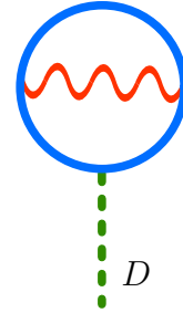
Figure 2: Diagram with gauge field insertion, proportional to \frac{e^2}{|\sigma|^2} .
