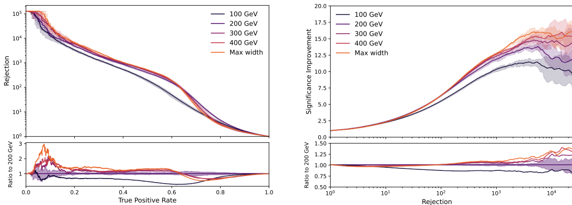
Figure 5: Background rejection as a function of signal efficiency (left) and significance improvement as a function of background rejection (right) for CURTAINS F4F trained with varying width side-bands, ranging from 100 GeV to the maximum width possible (SB1: 500 GeV, SB2: 900 GeV). All classifiers are trained on the sample with 3,000 injected signal events, using a signal region 3300 \leq m_{JJ} < 3700 GeV. The lines show the mean value of fifty classifier trainings with different random seeds with the shaded band covering 68% uncertainty.
