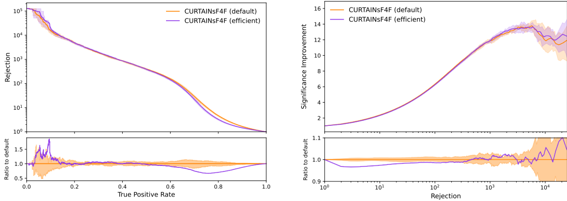
Figure 7: Background rejection as a function of signal efficiency (left) and significance improvement as a function of background rejection (right) for CURTAINS F4F using the default (orange) and efficient (purple) training configurations. All classifiers are trained on the sample with 3,000 injected signal events, using a signal region 3300 \leq m_{JJ} < 3700 GeV. The lines show the mean value of fifty classifier trainings with different random seeds with the shaded band covering 68% uncertainty.
