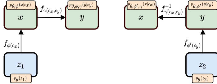
Figure 1: The Flows for Flows architecture for a conditional model [46]. Data x ( y ) are drawn from the initial distribution with conditional values c_x ( c_y ) and transformed to new values c_y ( c_x ) in a cINN f_\gamma(c_x, c_y) conditioned on c_x and c_y . The probability of the transformed data points are evaluated using a second normalizing flow for the base distribution f_{\phi'(c_y)} ( f_{\phi(c_x)} ). In the case where x and y are drawn from the same underlying distribution p(x, c) , the same base distribution f_\phi can be used.
