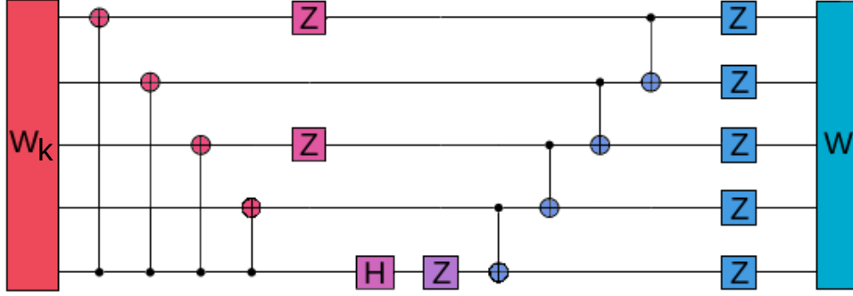
Figure 1: Pictorial representation of the Clifford circuit \hat{S} in (6) for L = 5 . The H and Z boxes stand respectively for the Hadamard gate and the \sigma^z operator on the chosen qubit. The CNOT gates involve two qubits and are represented by a line connecting a black dot, indicating the qubit that acts as the controller, and a colored circle signaling the one that can be flipped.
