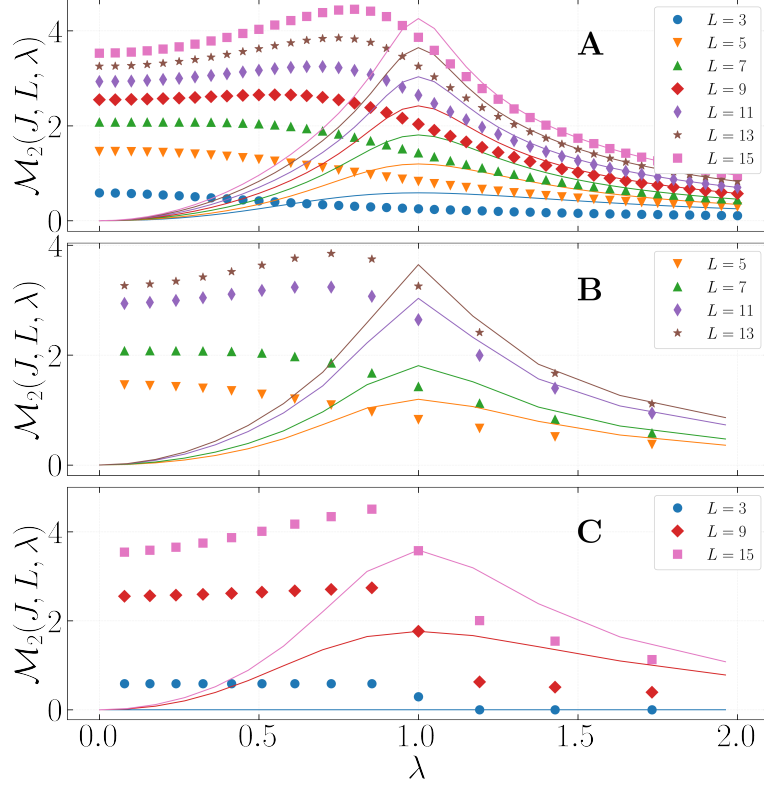
Figure 2: Behavior of the SRE as function of the parameter \lambda for the TFIM (Panel A), CIM with odd L not integer multiple of 3 (Panel B) and CIM with L odd and integer multiple of 3 (Panel C). In all panels the plots represent the value of SRE obtained for frustrated systems ( J = 1 ) while the lines depict the SRE for unfrustrated ones ( J = -1 ).
