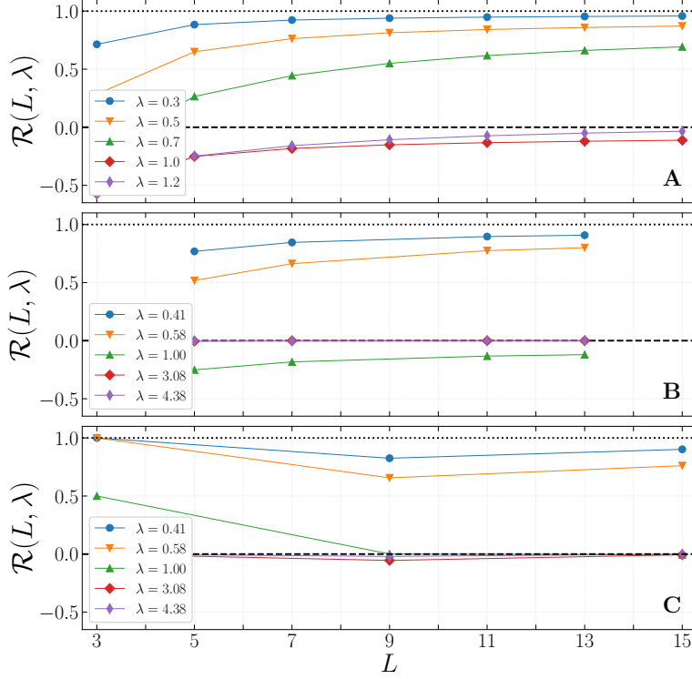
Figure 4: Behavior of the function \mathcal{R}(L, \lambda) in (8) as function of L for different models and values of \lambda : TFIM (panels A); CIM with L not an integer multiple of 3 (panels B); CIM with L an integer multiple of 3 (panels C).
