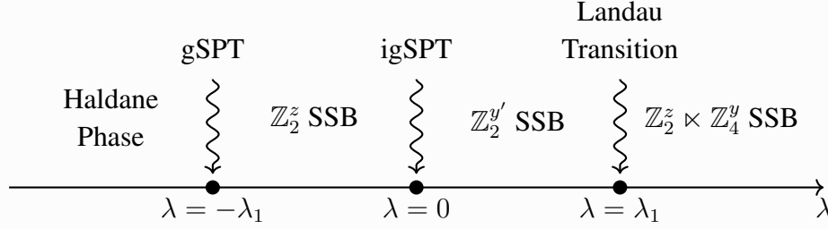
Figure 6: The phase diagram of (4.1) when \theta=0 .
