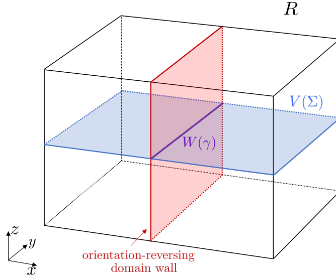
Figure 5: The configurations of the operators U(R), V(\Sigma), W(\gamma) that appear in the commutation relation Eq. (42).
