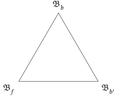
Figure 1: Triality between the triplet of bond algebras (6).
