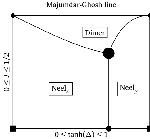
Figure 3: Phase diagram of Hamiltonian (80) in the reduced coupling space (82) with 0 \leq J \leq 1/2 . There are three phases: the \text{Neel}_x , the \text{Neel}_y , and the dimer phase. Each one of these three phases corresponds to gapped and two-fold degenerate ground states in the thermodynamic limit. In each phase, a non-degenerate ground state is selected by spontaneous symmetry breaking of the symmetry group G_{\text{tot}} defined in Eq. (59). The dimer phase is found on both sides of the open MG line defined by 0 < \Delta < \infty and J = 1/2 . All the phase boundaries with 0 < \Delta < \infty and J < 1/2 are continuous quantum phase transitions that realize deconfined quantum criticality [138]. The tricritical point (the large black circle) where the three phases meet realizes the \text{SU}(2)_1 conformal field theory in (1+1) -dimensional spacetime.
