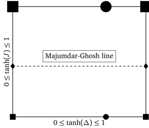
Figure 2: Exactly soluble points in the phase diagram of Hamiltonian (80) in the reduced coupling space (82). The small squares at the lower left and right corners of the phase diagram each realize the antiferromagnetic nearest-neighbor Ising chain. The large squares at the upper left and right corners of the phase diagram each realize two identical and decoupled antiferromagnetic nearest-neighbor Ising chains. The ground states are long-range ordered, gapped, and two-fold (four-fold) degenerate for the lower (upper) corners. The line (\Delta, J = 0) realizes non-interacting fermions without fermion-number conservation, except when \Delta = 1 . The small circle at (\Delta = 1, J = 0) realizes non-interacting spinless fermions at half filling with a nearest-neighbor uniform hopping amplitude. The ground state is gapless with a quantum criticality encoded by a c = 1 conformal field theory in (1 + 1) -dimensional spacetime in the thermodynamic limit. The large circle at (\Delta = 1, J = \infty) realizes two decoupled chains of non-interacting spinless fermions at half filling with a nearest-neighbor uniform hopping amplitude. The ground state is gapless with a quantum criticality behavior encoded by a c = 2 conformal field theory in (1 + 1) -dimensional spacetime in the thermodynamic limit. The diamonds at (\Delta, J) = (0, 1/2), (\infty, 1/2) are first-order boundaries between the phases governed by the Ising fixed points (small and large squares) at \Delta = 0 and \Delta = \infty , respectively. The open Majumdar-Ghosh (dashed) line at (\Delta, 1/2) with 0 < \Delta < \infty realizes the dimer phase. The dimer ground states are gapped and two-fold degenerate along the Majumdar-Ghosh (dashed) line.
