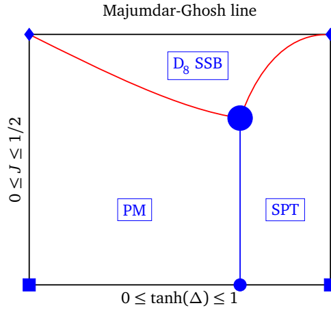
Figure 4: Phase diagram of Hamiltonian (88) with the Hilbert space \mathcal{H}_{b'=0}^{\vee} as domain of definition. The red boundaries realize a continuous quantum phase transition that separate two phases, one of which descends from the other through spontaneous symmetry breaking by which a symmetry-breaking local order parameter acquires a non-vanishing expectation value in the symmetry-broken phase, i.e., the Landau-Ginzburg paradigm of phase transitions. The blue boundary realizes a continuous topological quantum phase transition between two phases that are distinguished by a non-local order parameter. These phases are adiabatically connected to the ground states (90) and (91) for \Delta < 1 and \Delta > 1 , respectively.
