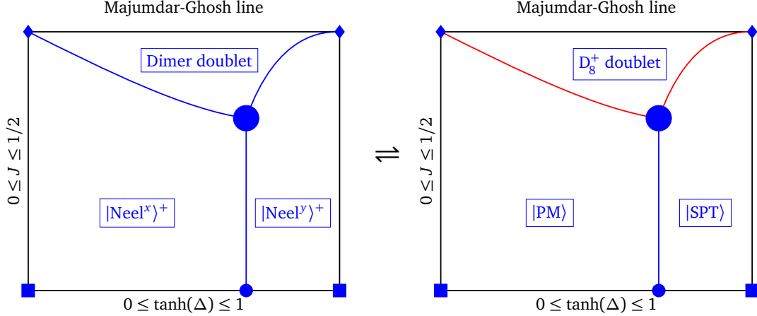
Figure 4: Phase diagram of Hamiltonian (88) with the Hilbert space \mathcal{H}_{b'=0}^{\vee} as domain of definition. The red boundaries realize a continuous quantum phase transition that separate two phases, one of which descends from the other through spontaneous symmetry breaking by which a symmetry-breaking local order parameter acquires a non-vanishing expectation value in the symmetry-broken phase, i.e., the Landau-Ginzburg paradigm of phase transitions. The blue boundary realizes a continuous topological quantum phase transition between two phases that are distinguished by a non-local order parameter. These phases are adiabatically connected to the ground states (90) and (91) for \Delta < 1 and \Delta > 1 , respectively.
