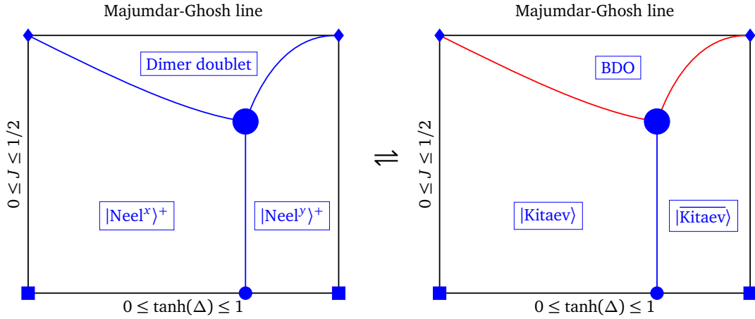
Figure 6: The phase diagram of Hamiltonian (80) restricted to the subspace \mathcal{H}_{b=0,+} of the Hilbert space \mathcal{H}_{b=0} is dual to the phase diagram of Hamiltonian (98) restricted to the subspace \mathcal{H}_{f=1,+}^V of \mathcal{H}_{f=1}^V . The pair of dual subspaces are to be found in the third line of Table 2. The two states |\text{Neel}^x\rangle^+ and |\text{Neel}^y\rangle^+ are defined in Eqs. (95) and (96), respectively, while the box “Dimer doublet” refers to the ground states (85c). On the dual side, the two non-trivial and distinct invertible topological states |\text{Kitaev}\rangle and |\overline{\text{Kitaev}}\rangle are defined in Eq. (100). The box “BDO” stands for the bond-density ordered phase described by the two-fold degenerate ground states (101) along the MG line. The symbols \rightarrow and \leftarrow denote gauging the diagonal subgroups generated by \widehat{U}_{r_\pi^z} and by its dual \widehat{P}_F^V defined in Eq. (73a), respectively.
