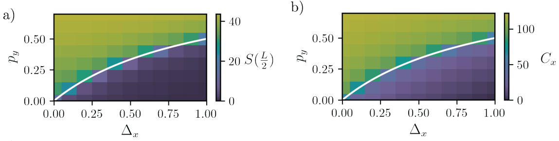
Figure 8: (a) Steady state half cut entanglement, S(x = L/2) , and (b) coherence, C_x , for the hybrid circuits with a sequence of random CNOTs and X , Y and Z measurements for the small measurement rate of p_m = 0.01 ( p_R = 0 and p_e = 0 ). In these figures \Delta_x parameterizes the imbalance between X and Z measurements \Delta_x = (p_x - p_z)/(1 - p_y) . These figures show the critical line (white), |\Delta_x| = p_y/(1 - p_y) , which is predicted by the competition between coherence loss and growth rates as discussed in the text. Due to the duality between the X and Z bases, dynamics are the same for \Delta_x \rightarrow -\Delta_x . For the \Delta_x > 0 side of the duality, the coherence in the Z basis, C_z , is greater than C_x and does not constrain the entanglement. These figures were computed with L = 128 and averaging over 2000 circuit realizations.
