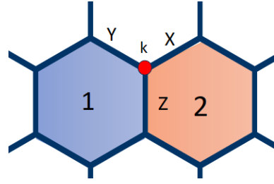
FIG. 3. Independent Gauss law constraints from hexagons 1 and 2.
