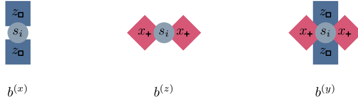
Figure 4: An illustration of the three different bond types b_i^{(\alpha)} with \alpha \in \{x, y, z\} . These bonds contain the respective charge and flux sites as well as the spin i which are affected by the action of Pauli matrices \sigma_i^x, \sigma_i^z and \sigma_i^y .
