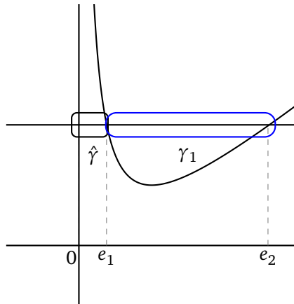
Figure 3. WKB loops for potential V = x + u_2/x
