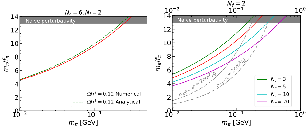
Figure 5. (left): Relic density contour obtained by numerically solving Boltzmann equation (red solid line) and corresponding analytical solution (green dashed line) for fixed N_C = 6, N_F = 2 . Relic density contours ( \Omega h^2 = 0.12 ) in m_\pi/f_\pi - m_\pi plane (solid lines) for various values of N_C and two Dirac fermions. Contours representing the DM self interaction cross section of 2 \text{ cm}^2/\text{g} are also shown if all 9 pions take part in the interaction (light green dot dashed line) or only neutral pions ( \tilde{\pi}^1, \tilde{\pi}^2, \tilde{\pi}^3 ) are accounted for (dashed dark green line).
