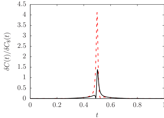
FIG. 2. The instantaneous energy cost against the standard instantaneous energy cost. The horizontal axis is time. The black solid curve represents a scheme with modulation \delta = 0.00427 and the red dashed curve represents that without modulation. Here, the energy gap is 2\Gamma_0 = 0.2 .
