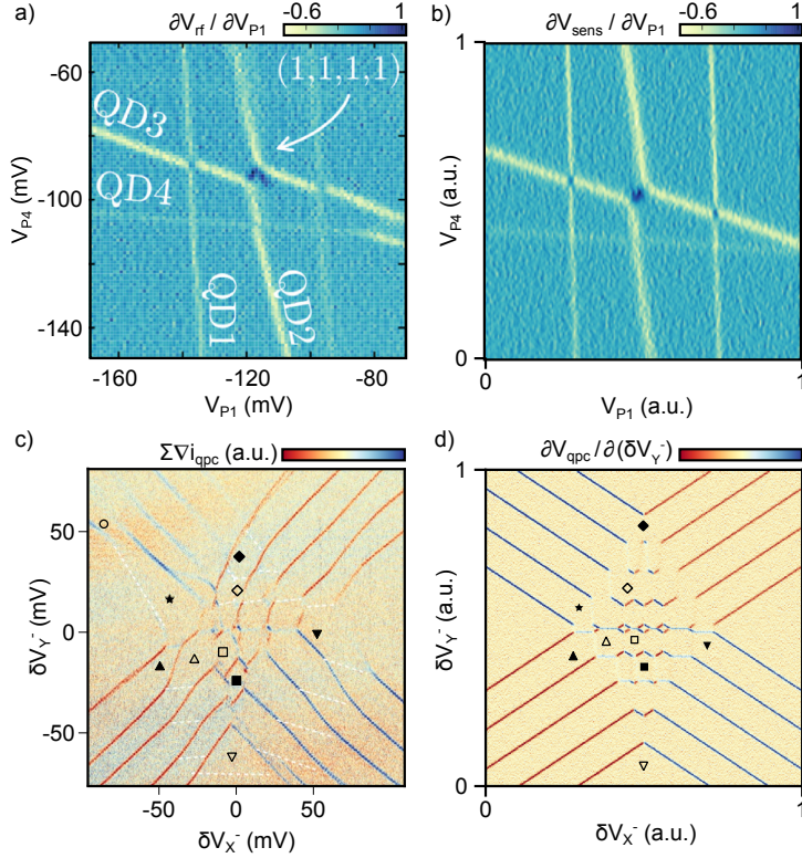
Figure 5. (a) Adaptation of Fig. 2b from Ref. [22] showing a stability diagram of a linear quadruple quantum dot array in the open regime. This is measured as a function of the two outermost plunger gates voltages, V_{P1} and V_{P4} . The colour scale represents the derivative of the sensor signal V_{rf} with respect to V_{P1} . (b) A recreation of Fig. 2b from Ref. [22], simulated using QArray. The colour scale represents the derivative of the simulated sensor signal, V_{sens} , with respect to V_{P1} . (c) Adaptation of Fig. 3a from Ref. [23] showing the stability diagram of a five-electron configuration corresponding to a five-dot cross-geometry array. The colour scale represents the sum of current changes in all charge sensors ( \sum \nabla i_{qpc} ) as a function of virtual gates \delta V_{X^-} (controlling the left-right detunings) and \delta V_{Y^-} (controlling the top-bottom detunings). (d) A recreation of Fig. 3a from [23] using QArray. The colour scale represents the derivative of the simulated sensor signal, in this case, V_{qpc} , with respect to \delta V_{Y^-} . To simulate the sensing of a QPC, we use the same method as in section IV A, using a linear profile instead of a Lorentzian one.
