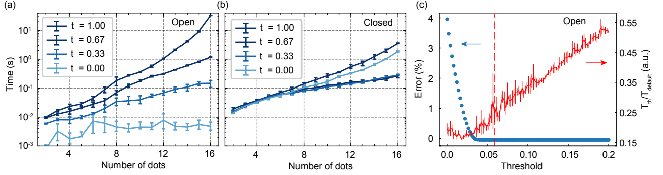
Figure 7. (a-b) Average computation time required by the Rust core to generate a 100 \times 100 pixels charge stability diagram computed with different threshold values for increasing numbers of quantum dots both for open and closed quantum dot arrays. The error bars denote the two standard deviation confidence intervals. (c) Comparison between the pixel values corresponding to the charge stability diagram of Fig. 5(b) computed with and without the threshold algorithm. The axis on the left is the percentage error obtained for the thresholded algorithm as a function of the threshold value. The axis on the right is the time saved when using the threshold algorithm. The error bars represent the standard deviation of the calculation time over 10 repetitions. The dashed line corresponds to an optimal threshold value that achieves a time save of a factor of 4 without introducing artefacts in the charge stability diagram.
