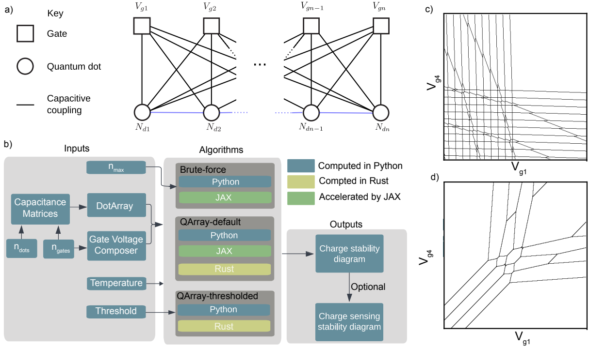
Figure 1. (a) Schematic of a generic array of quantum dots: The diagram illustrates the representation of a quantum dot device as a system of capacitively coupled electrostatic gates and quantum dots. Solid black lines represent the direct dot-to-gates couplings, while capacitors representing the interdot capacitance are modelled with blue lines, respectively. From the choice of the capacitance matrix (stored in the DotArray class), the user can define an array with an arbitrary number of dots and geometry. For given gate voltages, a discrete integer number of charges minimises the system’s free energy. (b) The structure of the QArray package featuring the multiple software implementations, represented as colour-coded boxes denoting Python (blue), Rust (yellow), and JAX (green), of the brute-force, default and thresholded algorithms. The gate voltage composer class generates voltage vectors for native sweeps (e.g., V_{g1} against V_{g2} ), or it can be used to define arbitrary virtual gate sweeps. DotArray offers methods for computing charge stability diagrams for open or closed regimes with any core choice. Optionally, the charge stability diagram can be coupled with simulated charge sensors to model their response. (c) Charge stability diagrams (computed with our default algorithm implemented in Rust) for a hole-based linear array of four quantum dots in the open regime. The black lines denote transitions separating regions in the charge stability diagram with a fixed dot occupation. (d) Charge stability diagrams (computed with our default algorithm implemented in Rust) for the same linear four-dot array of quantum dots in the closed regime where the total number of charges in the array is fixed to four.
