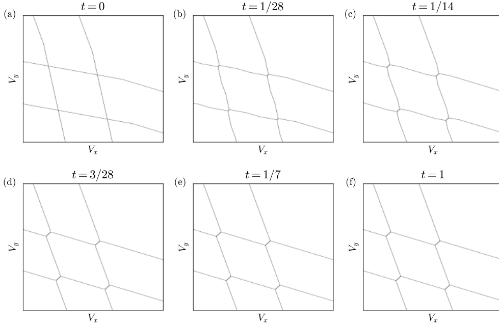
Figure 8. (a-e) Charge stability diagrams of an open double quantum dot produced by the thresholded algorithm for threshold values smaller than or equal to the empirical minimum value of 1/7 based on the capacitance matrix. The value of the threshold used in the simulation is stated above in the plot. f) Simulated charge stability diagram with the thresholded algorithm with the threshold set to one, so it performs identically to the default algorithm.
