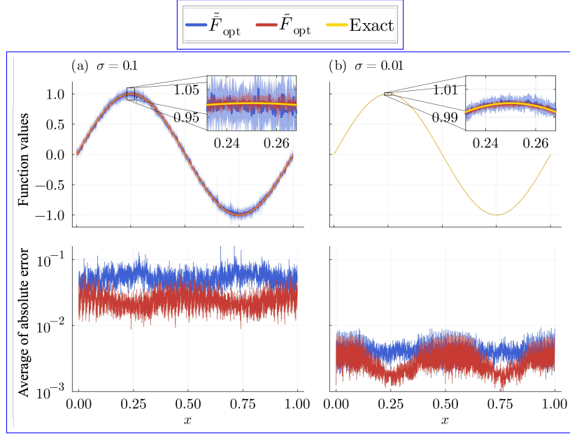
Figure 2: Results for our method applied to f_{\text{noise}}(x, \mu, \sigma) = f(x) \times (1 + N(\mu, \sigma^2)) with standard deviations \sigma = 0.1 and \sigma = 0.01 are shown in (a) and (b), respectively. In each figure, the upper panel shows the mean and variance across 20 runs, and the lower panel shows the mean of the absolute error. The insets within the upper panels provide magnified views of the region around x = 0.25 . Here, F_{\text{opt}} is the optimized QTT obtained after applying Step (b) (i.e., compressing the bond dimension to \chi = 2 before optimization), \tilde{F}_{\text{opt}} is the QTT optimized directly from the initial tensor with \tilde{\chi} = 6 , skipping Step (b), and “Exact” denotes the noise-free f(x) .
