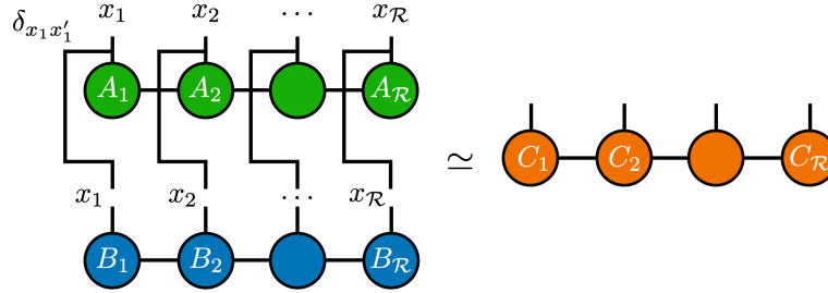
Figure 8: Diagram of the element-wise multiplication. The approximation means that the resulting TT is compressed by using SVD.
