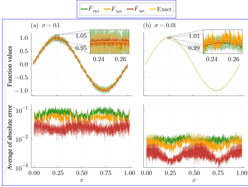
Figure 3: Results The setup and plotting same as in Fig. 2, but here we show results for our complete proposed method applied to f_{\text{noise}}(x, \mu, \sigma) = f(x) \times (1 + N(\mu, \sigma^2)) with standard deviations of the normal distribution \sigma = 0.1 and \sigma = 0.01 are shown in (a) and (b), respectively. The upper part panel shows the mean and variance of 20 runs, and the lower panel shows the mean of the absolute error. The small figures inside the plots in the upper panel are enlarged views of the region around x = 0.25 . \tilde{F}_{\text{itpl}} is the QTT from QTCI, \tilde{F}_{\text{init}} the QTT with the bond dimension compressed prior to optimization, \tilde{F}_{\text{opt}} the optimized QTT, and “Exact” the noise-free f(x) .
