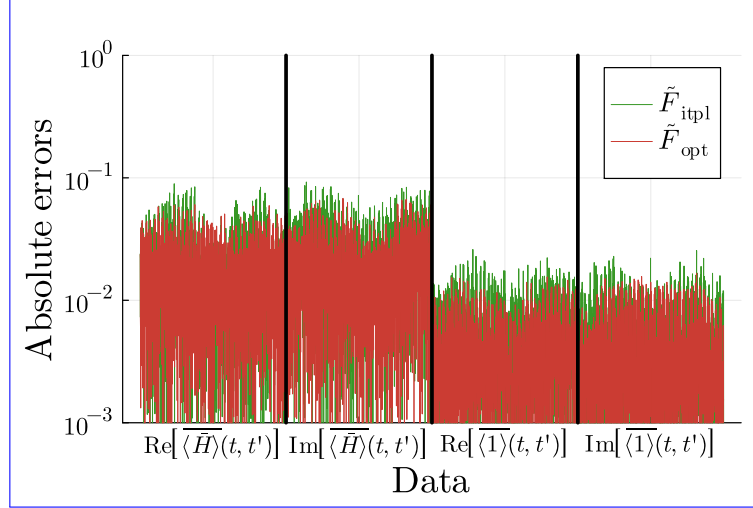
Figure 6: Results for the average absolute error between each of the values of the correlation function \langle \bar{H} \rangle(t, t') and \langle \bar{1} \rangle(t, t') obtained by applying the QTCI method (denoted as \tilde{F}_{\text{itpl}} ) or the proposed method (denoted as \tilde{F}_{\text{opt}} ) and the values from state vector simulation without noise. To enhance readability, we downsampled the displayed data to 1/50 of the original resolution. The average absolute error was calculated over 20 trials, each using a different set of random numbers. The presented results include the one-dimensional reshaped data series of function values that depend on t and t' . In both methods, for a system size of n_{\text{site}} = 4 , the parameters such as \lambda , \beta , \tau , T , \mathcal{R} , N_t , and M_s defined in Table 1 were used.
