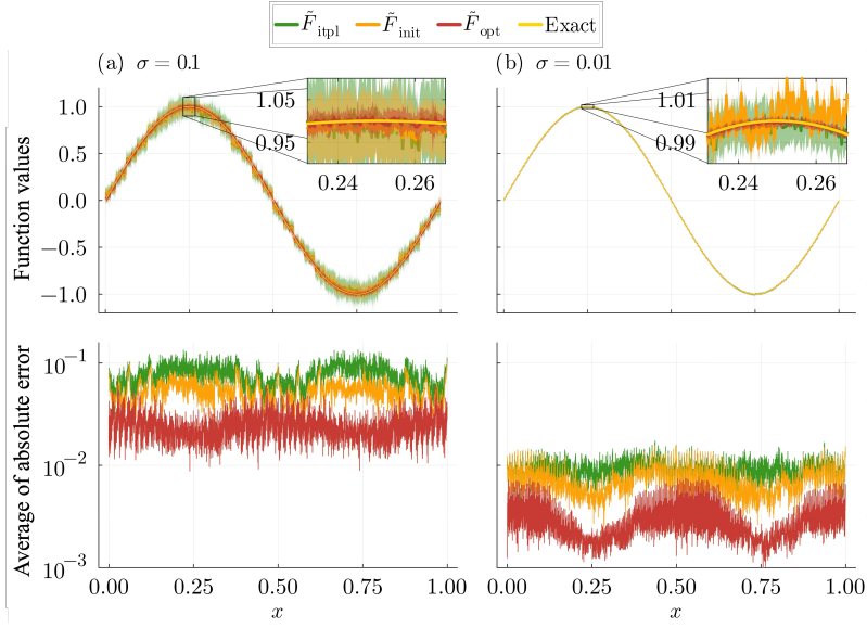
Figure 3: The setup and plotting same as in Fig. 2, but here we show results for our complete proposed method, including all three steps (a)–(c). \tilde{F}_{\text{itpl}} is the QTT from QTCI, \tilde{F}_{\text{init}} the QTT with the bond dimension compressed prior to optimization, \tilde{F}_{\text{opt}} the optimized QTT, and “Exact” the noise-free f(x) .
