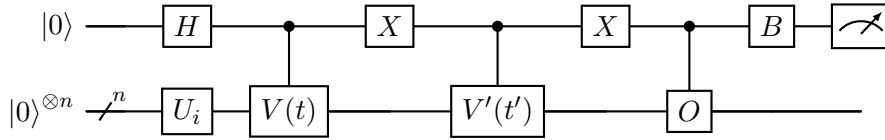
Figure 9: Quantum circuit for calculating \overline{\langle O \rangle}(t, t') . Here, we denote unitary operators V(t) = e^{-i\bar{H}t} , V'(t') = e^{-i\bar{H}t'} , and U_i = H^{\otimes n} , along with the unitary physical quantity O . Additionally, the B gate is set to B = H (Pauli- X measurement) for calculating the real part of \overline{\langle O \rangle}(t, t') , and B = HS^\dagger (Pauli- Y measurement) for calculating the imaginary part.
