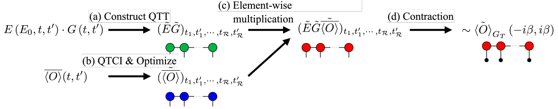
Figure 4: Calculating \langle \tilde{O} \rangle_{G_T}(-i\beta, i\beta) using our proposed method through following Steps. First, in Step (a), we construct (\tilde{E}\tilde{G})_{t_1, t'_1, \dots, t_{\mathcal{R}}, t'_{\mathcal{R}}} using the QTCI method. Next, in Step (b), we apply our proposed method to \overline{\langle O \rangle}(t, t') . Then, in Step (c), we perform element-wise multiplication of the QTTs obtained in Steps (a) and (b), resulting in (\tilde{E}\tilde{G}\overline{\langle \tilde{O} \rangle})_{t_1, t'_1, \dots, t_{\mathcal{R}}, t'_{\mathcal{R}}} . Finally, in Step (d), we integrate (\tilde{E}\tilde{G}\overline{\langle \tilde{O} \rangle})_{t_1, t'_1, \dots, t_{\mathcal{R}}, t'_{\mathcal{R}}} over the range of [-T, T] to compute \langle \tilde{O} \rangle_{G_T}(-i\beta, i\beta) .
