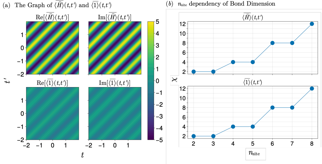
Figure 10: Computed correlation functions using state-vector simulation without shot noise, Trotter error (a), and their maximum bond dimensions (b). The QTT was constructed using SVD, setting its tolerance 10^{-10} .
