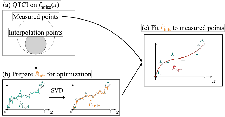
Figure 1: The optimization of TTs QTTs proposed in this study. In Step (a), we apply the QTCI to the function f_{\text{noise}}(\mathbf{x}) evaluated with random noise and store measured points obtained from QTCI. In Step (b), we build \tilde{F}_{\text{itpl}} , which is composed of interpolation points obtained from QTCI, where the triangle marks in (b) represent the interpolation points. This is then compressed by applying SVD to obtain an initial guess of QTT, \tilde{F}_{\text{init}} . In Step (c), we optimize the \tilde{F}_{\text{init}} by fitting it to the measured points obtained in Step (a) by applying the least squares method to reduce the effect of noise in \tilde{F}_{\text{init}} . This results in \tilde{F}_{\text{opt}} that approximate the noise-free function f(\mathbf{x}) .
