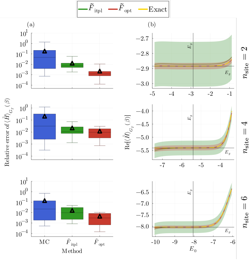
Figure 7: Results for the relative error of the ground-state energy computed by exact diagonalization method and each scheme (a) and E_0 dependency of the real part of the \langle \tilde{H} \rangle_{G_T}(\beta) (b). Here, we compute its variation over 20 calculations using each scheme, with each different random seed. The triangle markers in (a) and the solid line in (b) represent the mean values, and the shading indicates the variance. The parameter set used for implementation is presented in Sec. 5.2.4. Due to the high variance of the Monte Carlo results, they are omitted from Fig. 7(b).
