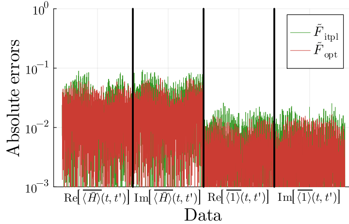
Figure 6: Results for the average absolute error between each of the values of the correlation function \langle \tilde{H} \rangle(t, t') and \langle \tilde{1} \rangle(t, t') obtained by applying the QTCI method (denoted as \tilde{F}_{\text{itpl}} ) or the proposed method (denoted as \tilde{F}_{\text{opt}} ) and the values from state vector simulation without noise. To enhance readability, we downsampled the displayed data to 1/50 of the original resolution. The average absolute error was calculated over 20 trials, each using a different set of random numbers. The presented results include the one-dimensional reshaped data series of function values that depend on t and t' . In both methods, for a system size of n_{\text{site}} = 4 , the parameters such as \lambda , \beta , \tau , T , \mathcal{R} , N_t , and M_s defined in Table 1 were used.
