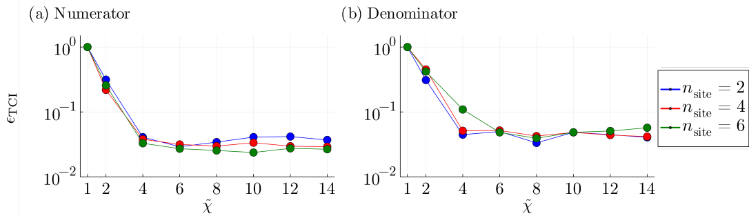
Figure 5: Normalized error \epsilon_{\text{TCI}} as a function of the bond dimension \tilde{\chi} for QTCI. (a) numerator \langle \bar{H} \rangle(t, t') , and (b) denominator \langle \bar{I} \rangle(t, t') . The parameters such as \lambda , \beta , \tau , T , \mathcal{R} , N_t , and M_s are set as in Table 1.
