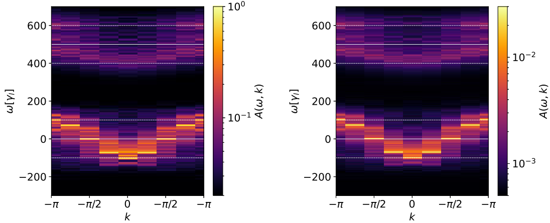
Figure 9: Spectral function A(\omega, k) of the Markovian open system dynamics in the NESS. Left: Under unitary dynamics (see Appendix G.5); Right: Under Lindbladian dynamics. The parameters are: U = 500\gamma_l , J = 50\gamma_l , z = 0.2 , L = 8 , N_s = 3 . The horizontal white lines are as in Fig. 5.
