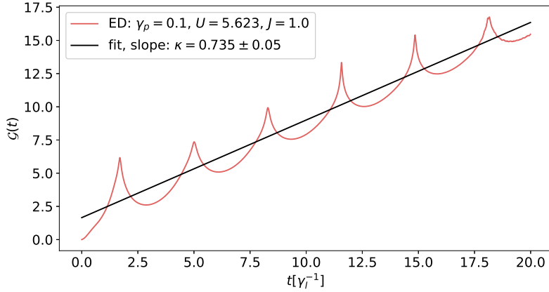
Figure 10: Logarithm of the retarded Green's function \mathcal{G}(t) = -\Re\left[\ln iG_{00}^R(t, 0)\right] (dimensionless) obtained from exact diagonalisation (red solid line), as a function of time (in units of \tau_l ) for the site j = 0 . Within the single-pole approximation, the decay rate is estimated by fitting \mathcal{G}(t) by a linear model. The result of the fit is shown as the black solid line. The parameters are U = 5.623\gamma_l , J = \gamma_l , z = 0.1 , L = 4 , N_s = 4 .
