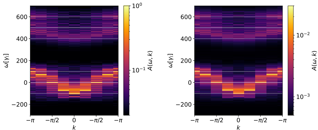
Figure 9: Spectral function A(\omega, k) of the temporal evolution in the NESS. Left: Under unitary dynamics (see Appendix G.5); Right: Under Lindbladian dynamics. The parameters are: U = 500\gamma_L , J = 50\gamma_L , z = 0.2 , L = 8 , N_s = 3 . The horizontal white lines are as in Fig. 5.
