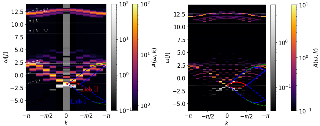
Figure 6: Spectral function A(k, \omega) for the ground state of the Bose-Hubbard model under unitary evolution (negative values in grey). The blue and red lines indicate the Lieb-I and Lieb-II branches respectively, the green branch is a feature of the lattice model, see text. Left panel: Exact diagonalisation solution without truncation in the local Hilbert space at finite interaction ( L = 12 , N = 2 particles, U/J = 10 ), compare with Appendix G.5. Right panel: Larger system size ( L = 24 , N = 6 , U/J = 10 , with N_s = 3 obtained with DMRG).
