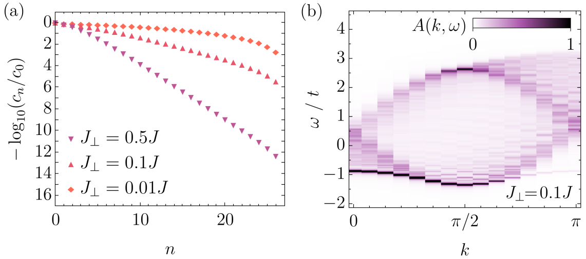
Figure 8: Properties of 1D t-J model (1) with a single hole and with added staggered magnetic field arising due to the coupling [ J_\perp/J in Eq. (15) in Appendix A] to neighboring chains in a quasi-1D geometry, cf. text and Appendix A. Panel (a) shows probabilities c_n of finding a configuration with n consecutive magnons attached to one side of the hole in the ground state of the respective model; panel (b) shows the spectral function A(k, \omega) calculated for the 1D t-J model with added staggered magnetic field J_\perp = 0.1J . All data obtained using exact diagonalization on a 28 sites periodic chain using J = 0.4t .
