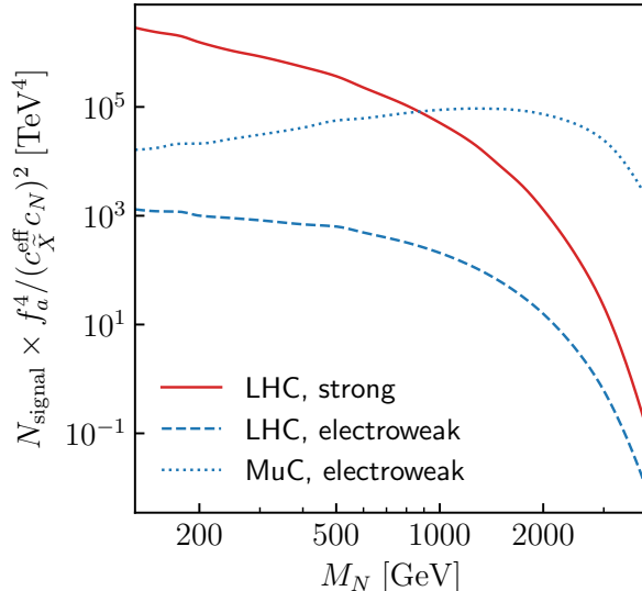
Figure 6: Expected number of signal events (excluding opposite-sign same-flavour processes) at the high-luminosity LHC ( 3 \text{ ab}^{-1} ) and a 10 TeV muon collider ( 10 \text{ ab}^{-1} ), normalized by the ALP couplings.
