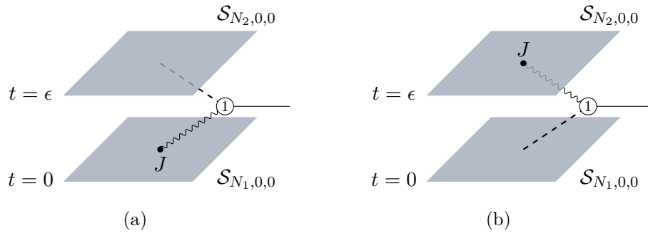
Figure 5: One-loop diagrams contributing to \Delta(T(z)) . The two surface defects \mathcal{S}_{N_1,0,0} and \mathcal{S}_{N_2,0,0} are located at t = 0 and t = \epsilon > 0 on \mathbb{R}_t , respectively. The limit \epsilon \rightarrow 0 is taken to initiate the fusion.
