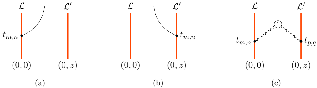
Figure 3: Feynman diagrams for fusion of line defects. The two line defects \mathcal{L} and \mathcal{L}' are located at (0, 0) and (0, z) on the holomorphic planes \mathbb{C}_x \times \mathbb{C}_z , respectively.
