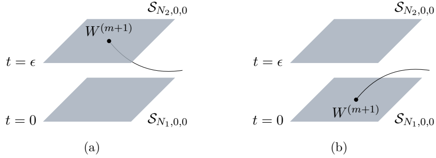
Figure 4: Tree diagrams for fusion of surface defects
