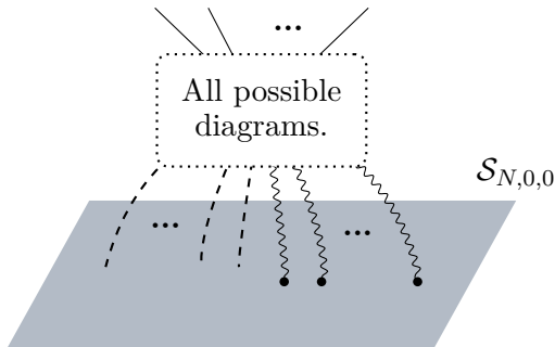
Figure 2: A generic diagram coupling the chiral defect \mathcal{S}_{N,0,0} to the 5d CS theory.
