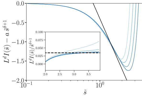
Figure 3: Rate function with its leading power law behavior subtracted, L^d I(\tilde{s}) - a \tilde{s}^{\delta+1} , as a function of \tilde{s} = L^{\beta/\nu} s , obtained from Monte Carlo simulations of the 3D Ising model of size L = 16, 32, 64, 128 (from light to dark blue) at criticality. The black line corresponds to -\frac{\delta-1}{2} \log(\tilde{s}) (note the log-scale of the abscissa). Inset: I(\tilde{s})/\tilde{s}^{\delta+1} as a function of \tilde{s} (linear scale). The dashed line corresponds to the constant a \simeq 0.034 extrapolated to infinite system size.
