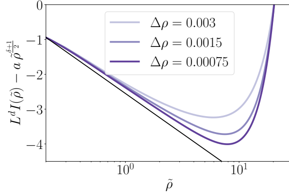
Figure 6: Subleading behavior of the rate function as a function of \tilde{\rho} = L^{2\beta/\nu} \rho from FRG for n = 1 for various grid mesh of the field \Delta\rho , keeping the maximum range \rho_M = 0.6 fixed. The black line shows the expected -\frac{\delta-1}{2} \log \tilde{\rho} . Decreasing the \Delta\rho allows for seeing the log behavior for larger and larger fields.
