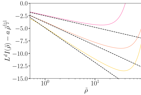
Figure 2: Rate function of the three-dimensional O(n) model with its leading powerlaw behavior subtracted, L^d I(\tilde{\rho}) - a \tilde{\rho}^{\frac{\delta+1}{2}} , as a function of \rho , obtained from FRG for n = 1, 2, 3 (top to bottom). Here \rho = s^2/2 and \tilde{\rho} = L^{2\beta/\nu} \rho , with 2\beta/\nu = (d-2) and \delta = 2d/(d-2) at LPA. The dashed lines correspond to -n \frac{\delta-1}{4} \log(\tilde{\rho}) (note the log-scale of the abscissa).
