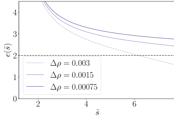
Figure 7: Estimator e(\tilde{s}) , Eq. (A.2), as a function of \tilde{s} for FRG at LPA and n = 1 . Same data as in Fig. 6. Depending on the mesh size \Delta\rho , the estimator can overshoot the predicted plateau at \psi = \frac{\delta-1}{2} (equal to 2 at LPA, shown as red dashed line). Decreasing \Delta\rho improves the behavior of e(\tilde{s}) .
