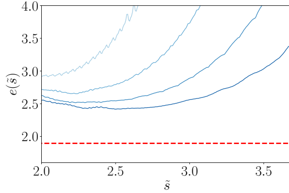
Figure 8: Estimator e(\tilde{s}) , Eq. (A.2), as a function of \tilde{s} from MC data for L = 16, 32, 64, 128 from light to dark blue. The dashed line corresponds to \psi = \frac{\delta-1}{2} . Finite-size corrections are still rather strong even for L = 128 , while the maximum range accessible in \tilde{s} is also rather limited and might not be yet in the deep universal rare event regime.
