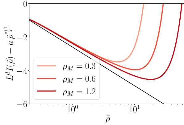
Figure 5: Subleading behavior of the rate function as a function of \tilde{\rho} = L^{2\beta/\nu} \rho from FRG for n = 1 for various maximum ranges of the field \rho_M , keeping the grid mesh \Delta\rho = 0.00075 fixed. The black line shows the expected -\frac{\delta-1}{2} \log \tilde{\rho} . Increasing the \rho_M allows for seeing the log behavior for larger and larger fields.
