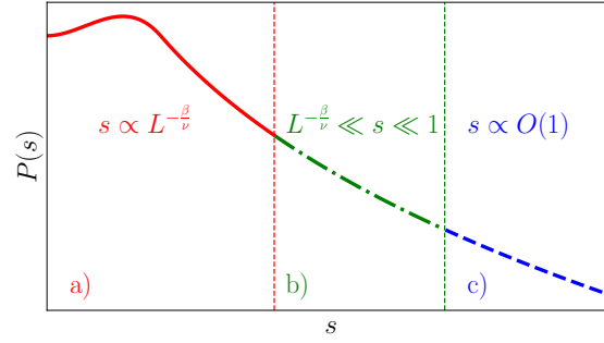
Figure 1: Schematic representation of different regimes of the probability distribution function of an O(n) critical system. The regime a) is the scaling regime where the probability distribution is a universal function of sL^{\beta/\nu} . This regime corresponds to a generalization of the CLT to strongly correlated variables. The universal large deviation regime b) appears for sL^{\beta/\nu} \gg 1 , where the PDF takes the form Eq. (1). This region is the main focus of the present work. Finally, regime c) is the non-universal large deviation regime. The cross-over from b) to c) is characterized by universal corrections to scaling multiplied by non-universal amplitudes, see Sec. 4.
