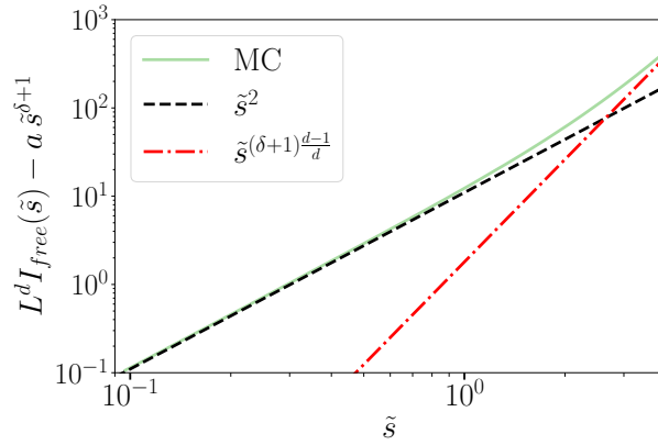
Figure 4: Rate function obtained from Monte Carlo simulations for the 3d Ising with L = 64 at T_c , but with free boundary conditions. Note that we have subtracted the same leading contribution a\tilde{s}^{\delta+1} that we found for periodic boundary conditions (shown in Fig. 3). The dashed line corresponds to a quadratic behavior at small magnetization, while the dotted-dashed line corresponds to a surface correction term.
