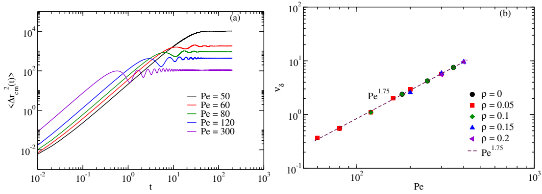
Figure 9: a) Mean-squared-displacement (MSD) of the end monomer with respect to the center of mass of the filament for various Pe at a given \rho = 0.05 . b) The rotation frequency is computed from oscillations of the MSD of the monomers for various \rho . The dashed line represents the power-law variation of the frequency \nu_\delta \sim Pe^{7/4} .
