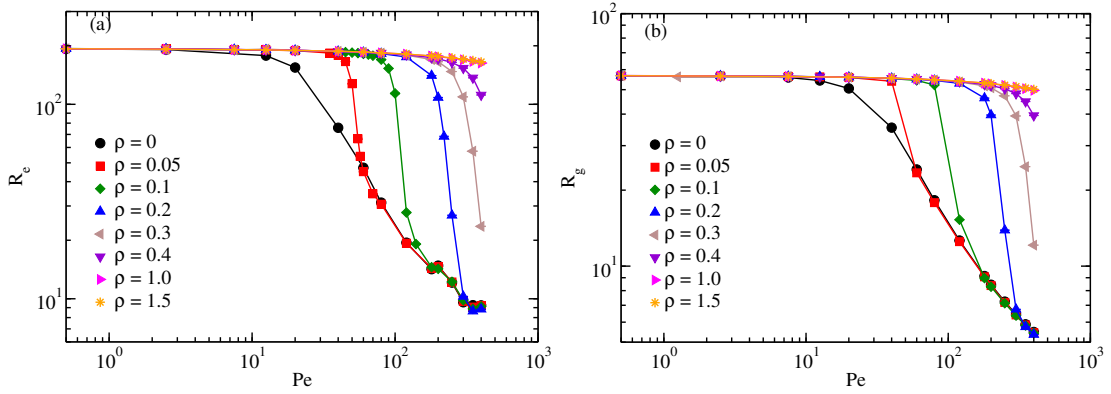
Figure 5: a) The variation of the average end-to-end distance R_e as a function of Péclet number Pe . b) The average radius of gyration R_g of the filament as a function of Péclet number Pe for various \rho as displayed in the plot.
