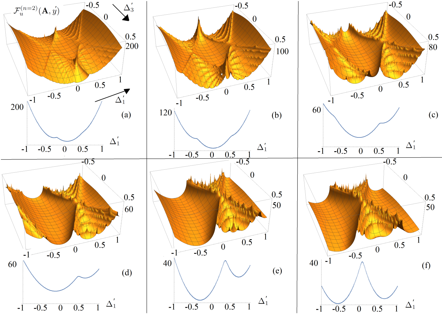
FIG. A6. \mathcal{F}_u^{(2)} in the dual space given in Eq. H3 for the Ising model with h = 0 , L = 10 , and m = -\sqrt{u - u} in terms of \Delta_1 and \Delta_3 for various rates of u : (a) u = 0.1 , (b) u = 0.2 , (c) u = 0.35 , (d) u = 0.5 , (e) u = 0.75 , and (f) u = 0.99 . We see that for 0.5 \lesssim u a second peak appears which makes the MF approximation questionable.
