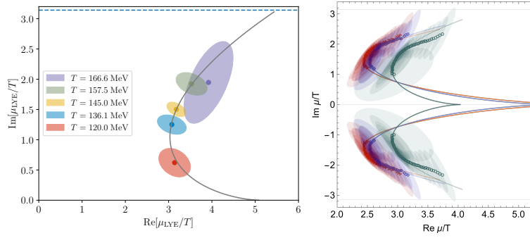
Figure 12: Left panel: the figure is from Ref. [54]. It shows the location of the Yang-Lee edge singularity as a function of temperature for N_\tau = 6 extracted using the imaginary baryon chemical potential data. The solid line is the result of the best fit with Eq. (68). Right panel: the figure is from Ref. [53]. In the figure, the location of the Yang-Lee edge singularity is displayed as a function of temperature extracted from Taylor series coefficients for N_\tau = 8 . The Yang-Lee edge locations (data points) and corresponding fits (solid lines) correspond to different extraction methods. The red triangles and the blue diamonds are obtained by utilizing two different conformal maps with subsequent Padé approximation. The green circles are obtained by using Padé without any conformal map.
