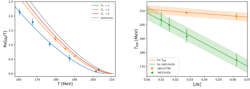
Figure 10: Left panel: scaling of the Yang-Lee singularity with temperature for three different lattice spacings ( N_\tau ) and continuum extrapolation, see Refs. [50, 51] for details. Right panel: the N_\tau dependence of the Roberge-Weiss transition temperature T_{RW}(N_\tau) from Refs. [50, 51] and direct calculation of Ref. [52].
