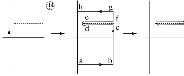
Figure 18: Computation of the Fourier coefficient for the function with one singularity in the right half-plane of complex baryon chemical potential. The figure is from Ref. [58].
