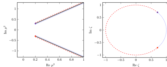
Figure 13: Illustration of the “two-cut” map of Ref. [53].
