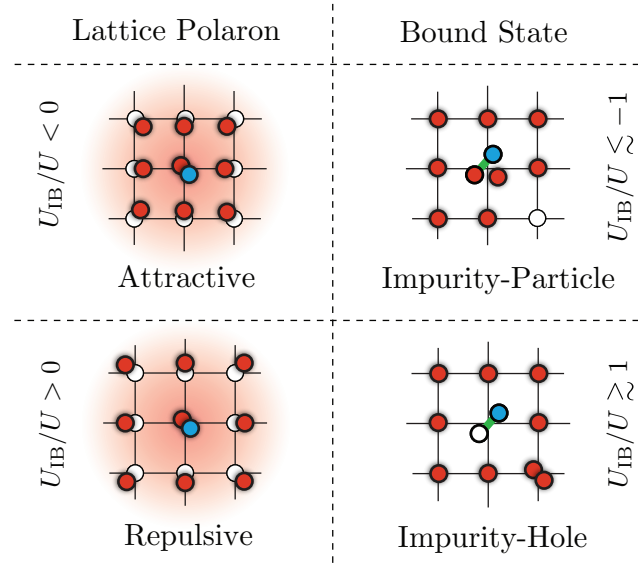
Figure 3: For U_{\text{IB}} < 0 , the impurity (blue) attracts the surrounding bosons (red) forming an attractive polaron. For U_{\text{IB}}/U \lesssim -1 , it forms a bound state with one extra boson. For U_{\text{IB}} > 0 , the impurity repels the surrounding bosons forming a repulsive polaron. For U_{\text{IB}}/U \gtrsim 1 , it pushes away the bosons completely forming a bound state with a hole.
