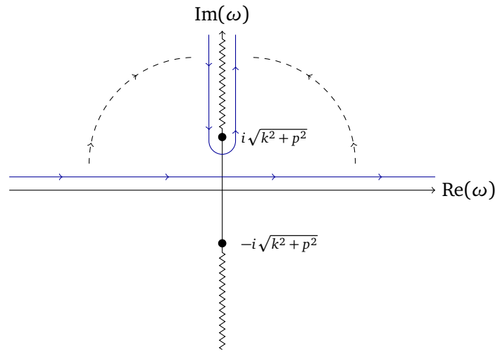
Figure 3: The contour deformation yielding the integral (A.5).
