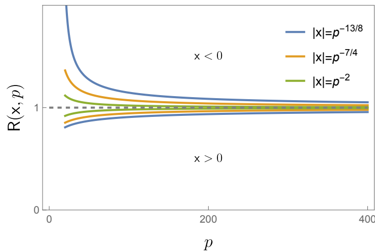
Figure 2: Numerical plots of R(x, p) for large p . Since x \sim N^{-2} each plot corresponds to p \sim N^\alpha with 1 < \alpha < \frac{4}{3} (specifically \alpha = 1, \frac{8}{7}, \frac{16}{13} , from bottom to top in the legend, respectively). When x > 0 the R approaches 1 from below while when x < 0 , it approaches 1 from above.
