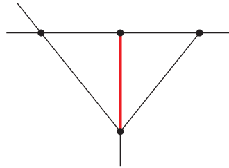
Sector 94, Topo \tilde{B}
