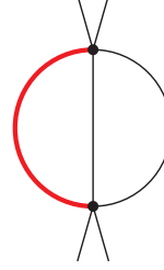
Sector 84, Topo \tilde{C}
