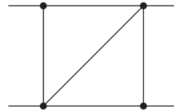
Sector 59, Topo \tilde{E}
