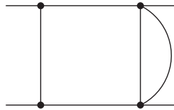
Sector 55, Topo \tilde{A} , \tilde{C} , \tilde{E}
