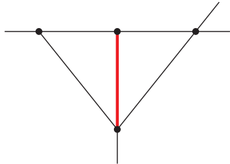
Sector 79, Topo E
