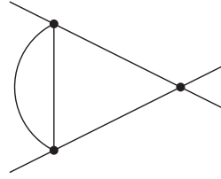
Sector 71, Topo B
