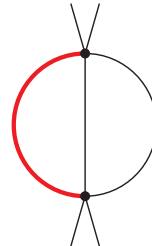
Figure 4: Master sectors for planar double-box integrals (part 1).
