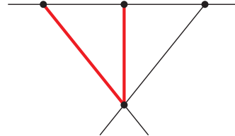
Sector 91, Topo \tilde{B}
