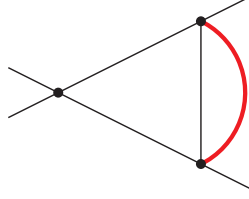
Sector 85, Topo \tilde{B}
