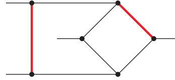
Sector 127, Topo \tilde{B}
