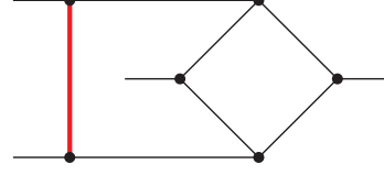
Sector 127, Topo \tilde{B}
