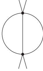
Sector 73, Topo \tilde{A}, \tilde{B}
