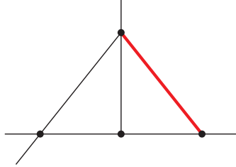
Sector 110, Topo \tilde{B}
