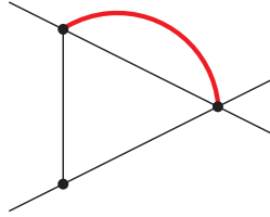
Sector 85, Topo \tilde{B}
