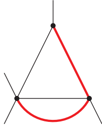
Sector 55, Topo B, D
