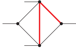
Sector 121, Topo \tilde{B}
