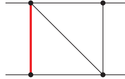
Sector 93, Topo B
