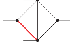
Sector 121, Topo \tilde{A}
