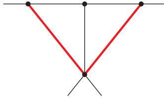
Sector 93, Topo E
