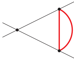
Sector 78, Topo A
