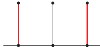
Sector 127, Topo B
