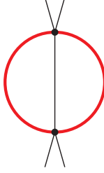
Sector 84, Topo \tilde{B}
