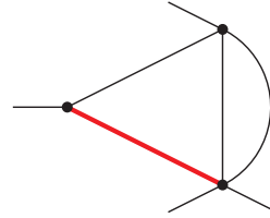
Sector 89, Topo \tilde{A}
