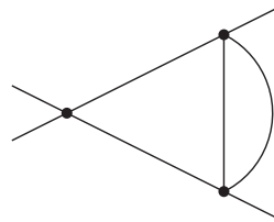
Sector 78, Topo D
