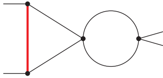
Sector 55, Topo B, D
