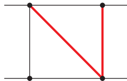
Sector 93, Topo A
