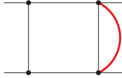
Sector 79, Topo \tilde{C}
