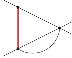
Sector 43, Topo \tilde{B}, \tilde{D}
