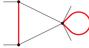
Sector 78, Topo D
