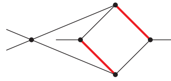
Sector 126, Topo \tilde{A}
