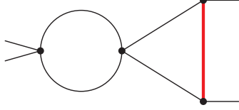
Sector 121, Topo A
