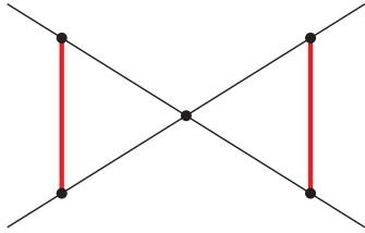
Sector 119, Topo B
