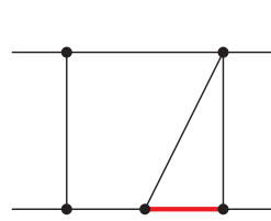
Sector 63, Topo \tilde{A}, \tilde{C}
