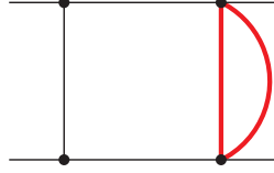
Sector 91, Topo B
