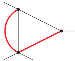
Sector 89, Topo A
