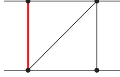
Sector 61, Topo \tilde{A} , \tilde{C}
