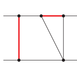
Sector 119, Topo \tilde{B}
