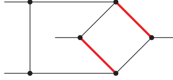
Sector 127, Topo \tilde{A}
