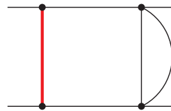
Sector 79, Topo D
