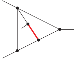
Sector 126, Topo \tilde{D}, \tilde{E}
