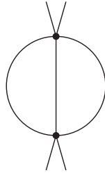
Figure 10: Master sectors for non-planar double-box integrals (part 1).
