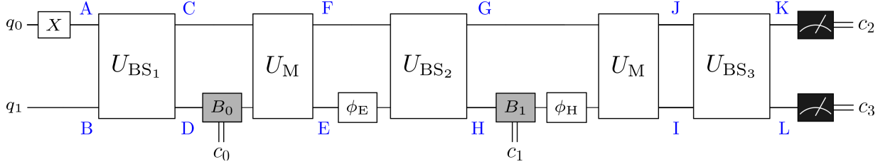
Figure 6: Quantum circuit for the modified Unruh's experiment. The state of qubits q_0 and q_1 correspond to the states of horizontal (A, C, F, G, J, K) and vertical (B, D, E, H, I, L) modes, respectively. The initial state prior to U_{BS1} is |\psi_0\rangle = |1\rangle_A |0\rangle_B , with the X gate required to initiate mode A as occupied. The double lines denoted by c_0 and c_1 represent the classical bits storing the results registered by the blockers B_0 and B_1 , respectively, and c_2 and c_3 by the detectors D_0 and D_1 , respectively.
