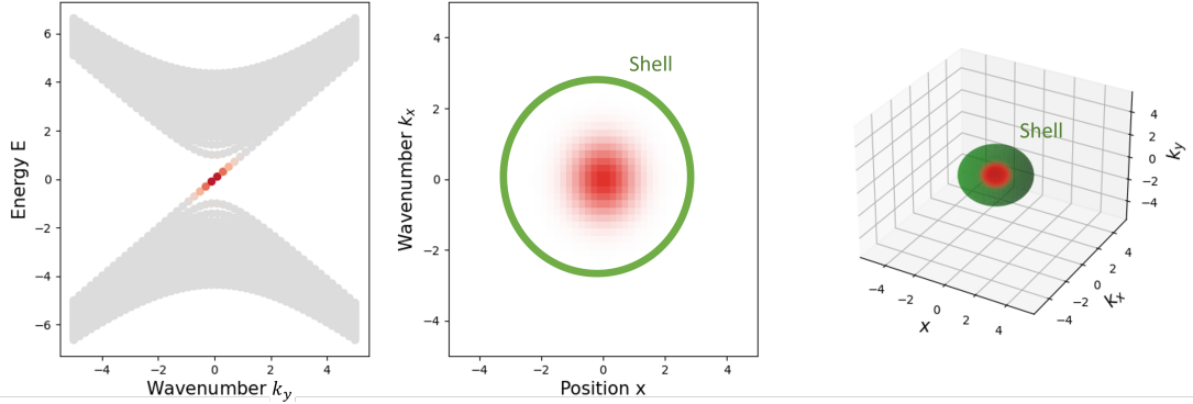
Figure 10: Numerical computation of the modified Jackiw-Rebbi model (25). (Left) Dispersion relation in k_y of the eigenstates of \hat{H}(k_y) . Modes are colored in red if they are both close to the Fermi energy E = 0 and located close to x = 0 , in grey otherwise. (Center) Wigner-Weyl transform of the gapless mode of \hat{H}(k_y) in k_y = 0 , the intersection of the shell for k_y = 0 is denoted in green. (Right) Wigner-Weyl transform of the modes of \hat{H}(k_y) of energy close to the Fermi-energy. The shell is a sphere and is displayed in green.
