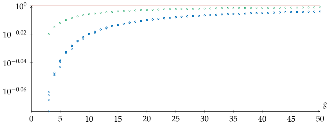
Figure 7: The 2-point correlators, normalised by their leading asymptotics: note the convergence to 1 + O(g^{-1}) . Also observe the differing convergence behaviour of the correlators with a \tau_0 insertion (in green) versus without (in blue); this suggests that the subleading terms do depend on the partition (d_1, \dots, d_n) . This is indeed the case, and it can be proved via resurgence.
