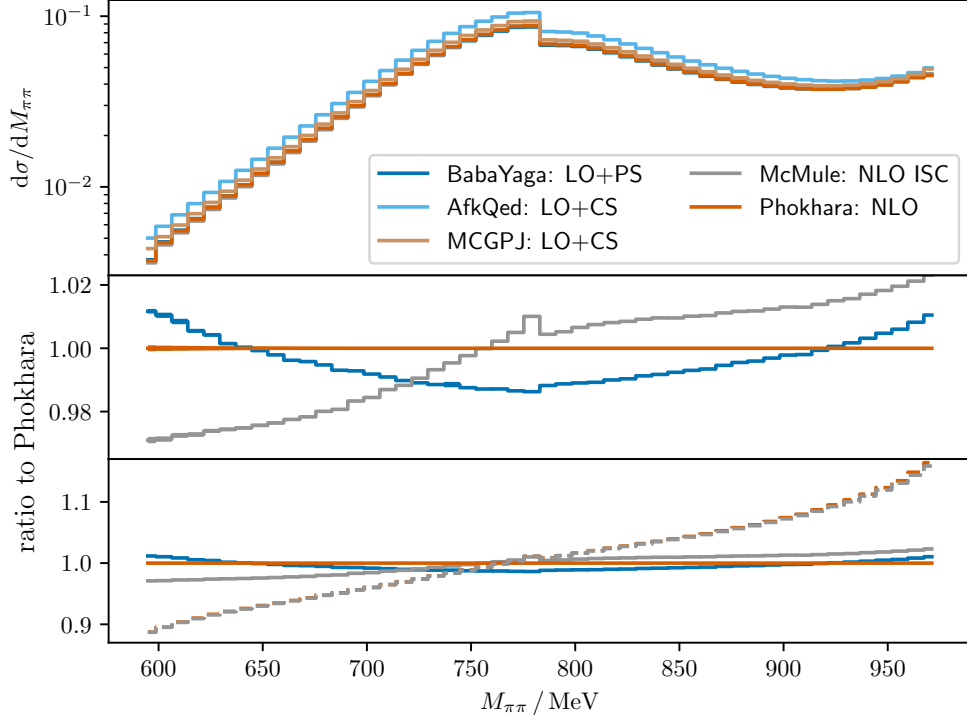
Figure 27: Distribution of M_{\pi\pi} in the KLOE-like small-angle scenario for e^+e^- \rightarrow \pi^+\pi^-\gamma . The dashed lines are the LO results, with (PHOKHARA) and without (MCMULE) final-state photon emission.
