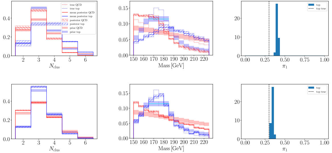
Figure 7: Number of clusters, mass and the probability of top jets distributions for the model with (bottom row) and without (upper row) correlations with \Sigma = 1400 . See text for the details.
