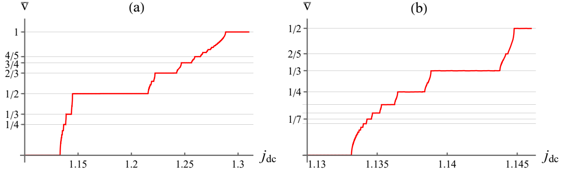
Figure 1: CVC of the Josephson junction with second Josephson harmonic in the CPR at j_{ac} = 0.8 , j_1 = 1 , and A = 0.7 . (a) Range of voltages below the first Shapiro step. Many fractional steps besides half-integer one are seen. (b) Range of voltages below the 1/2 Shapiro step [zoomed part of plot (a)]. Series of steps of type 1/k with k > 1 and the 2/5 step, which is part of 2/k series are seen. Amplitude of the 2/5 step is much less than amplitude of the steps of type 1/k .
