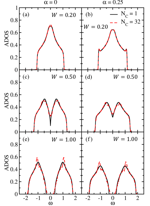
FIG. 1. ADOS computed using DCA for disordered two-dimensional electronic systems without Rashba SOC (left panels) and with SOC at \alpha = 0.25 (right panels). Panels (a)–(f) compare results for N_c = 1 (CPA, solid curves) and N_c = 32 (dashed curves) at increasing disorder strengths: W = 0.20 ((a), (b)), W = 0.50 ((c), (d)), and W = 1.00 ((e), (f)).
