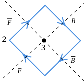
Figure 17: This figure is the 1 \leftrightarrow 2 version of the previous figure. We depict the motion of the insertion of the operator 2 for the sequence of moves F\bar{B}B\bar{F} acting on (P_{12}^{m_1, 0}, Q_{21}^{\bar{m}_1, -1}) . We start at the left corner of this diagram. The operations, \bar{F} , B , \bar{B} and F then respectively move us along the legs of this diamond. The total monodromy vanishes.
