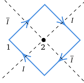
Figure 15: Illustration of the sequence of moves I\bar{I}I\bar{I} in a situation in which the monodromies associated with the two I moves add with each other, but are cancelled by the monodromies associated with the two \bar{I} moves (which also add with each other). The two I monodromies add rather than cancelling because while the top right I move cuts a future lightcone of 2, the bottom left I move cuts a past lightcone of 2 in the reverse direction. A similar analysis is applied for the move \bar{I} . The phases associated with I motion cancel the phases associated with \bar{I} motion because h - \bar{h} is an integer for all operators.
