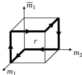
Figure 18: A closed contour in the lattice of causal configurations, which we decompose into a product of simple contours in two inequivalent ways in the next figure.
