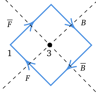
Figure 16: In this figure, we depict the motion of the insertion of the operator 1 for the sequence of moves F\bar{B}B\bar{F} acting on (P_{21}^{0, m_2}, Q_{12}^{-1, \bar{m}_2}) . We start at the left corner of this diagram. The operations, \bar{F} , B , \bar{B} and F then respectively move us along the legs of this diamond. As we explain in the main text, the total monodromy along this path also is zero.
