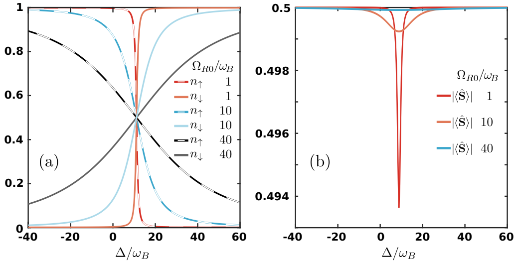
Figure 2: Description of Rabi-coupled polarons in terms of a two level model and its limitations. (a) Population of the spin- \uparrow and spin- \downarrow states and (b) expectation values of the spin-magnitude |\langle \hat{S}_\mu \rangle| for varying detuning \Delta and for N_I = 1 at different Rabi-couplings \Omega_{R0} (see legend). The polaronic (non-interacting) impurity states are reproduced for \Delta \rightarrow -\infty ( \Delta \rightarrow \infty ). For \Delta \approx -E_{1\uparrow}/\hbar , a correlated superposition state is created.
