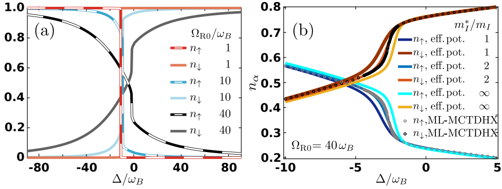
Figure 8: (a) Population of the spin- \uparrow and spin- \downarrow impurity states with respect to the detuning \Delta at different \Omega_{R0} (see legend) and within the strongly interacting case g_{BI} = 3g_{BB} = 1.5\sqrt{\hbar^3\omega_B/m_B} . The sharp transition for small \Omega_{R0} becomes gradually smoother and shifts as \Omega_{R0} increases. (b) Comparison of the ML-MCTDHX data for \Omega_{R0} = 40\omega_B with the effective potential for Z_{\text{eff}} = 1 and varying m_I^* (i.e. without fitting parameters). The excellent agreement of the corresponding data leads to the conclusion that the effective mass of the polaron within ML-MCTDHX is m_I^* = 2m_I . Notice that the range of \Delta values is restricted such that the deviations of n_\alpha between different values of m_I^* are better visible.
