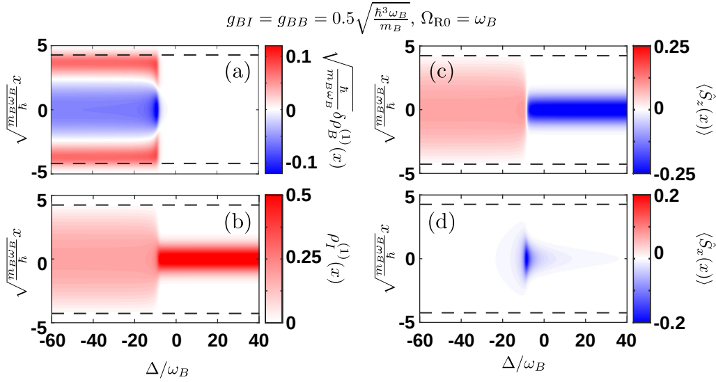
Figure 6: Behavior of the bath and impurity densities in the repulsive polaron case for critical interaction, g_{BI} = g_{BB} = 0.5 \sqrt{\hbar^3 \omega_B / m_B} , in terms of the miscibility-immiscibility transition and \Omega_{R0} = \omega_B . (a) Density fluctuations of the BEC background, \delta\rho_B^{(1)}(x) with respect to \Delta/\omega_B . (b) The total (spin-unresolved) impurity density \rho_I^{(1)}(x) in terms of \Delta . Spatially resolved expectation values of the spin operators (c) \hat{S}_z(x) and (d) \hat{S}_x(x) for varying \Delta . Superposition states of the impurity manifest by the \langle \hat{S}_x(x) \rangle < 0 regions in (d). The dashed lines mark the Thomas-Fermi radius of the BEC.
