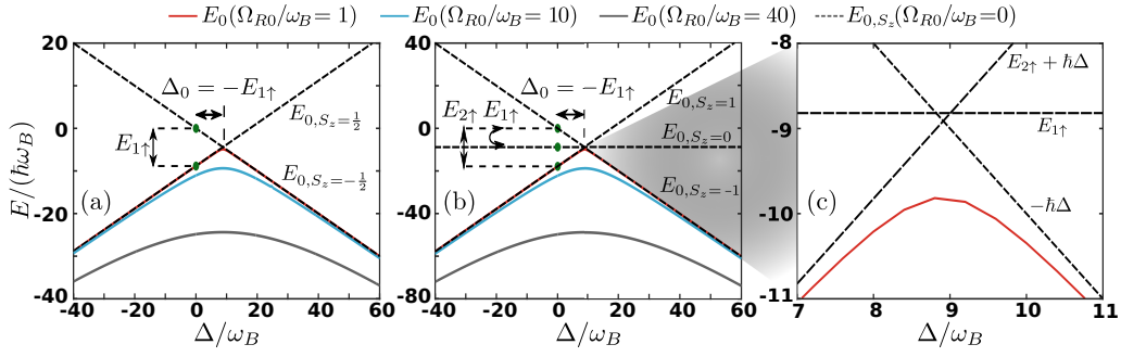
Figure 1: Ground state energies of Eq. (1) for (a) N_I = 1 and (b) N_I = 2 impurities with g_{BI} = -g_{BB} = -0.5 \sqrt{\hbar^3 \omega_B / m_B} and varying \Omega_{R0} (see legend). The dashed lines indicate the lowest in energy eigenstates for different S_z and \Omega_R = 0 . The important energy scales, E_{1\uparrow} , E_{2\uparrow} and \Delta_0 are also schematically illustrated. (c) Magnification of panel (b) in the vicinity of \Delta = -E_{1\uparrow} , highlighting the difference in energy between E_{2\uparrow} and 2E_{1\uparrow} .
