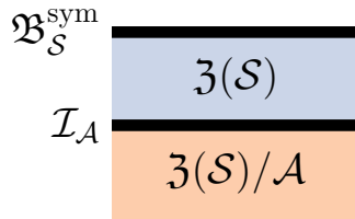
Figure 3: The classification of quantum phases characterized by a symmetry \mathcal{S} using the SymTFT \mathfrak{Z}(\mathcal{S}) is based on interfaces \mathcal{I}_{\mathcal{A}} with condensable algebras \mathcal{A} of the SymTFT. See Appendix A for an introduction.
