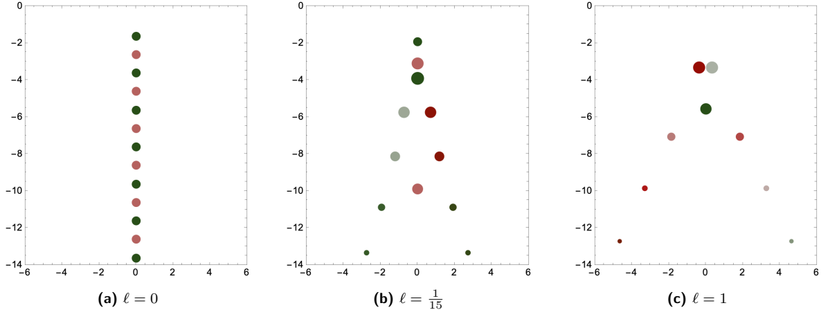
Figure 7: The quasinormal modes for the model (5.2) in the background f(r) = r^2 - 1 - \ell/r^2 + \ell/(4r^4) for various values of \ell . At \ell = 0 the residues grow too fast to be plotted in a useful way, so we choose a constant point size instead.
