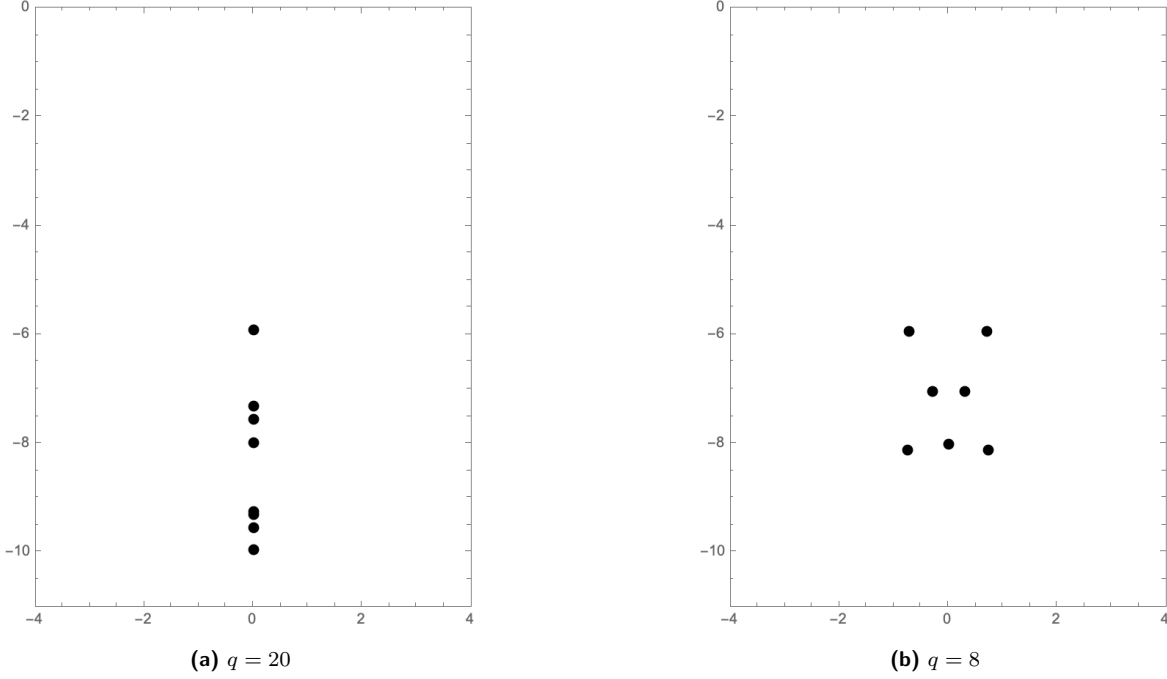
Figure 8: Converged zeroes of the spectral density for two different values of q .
