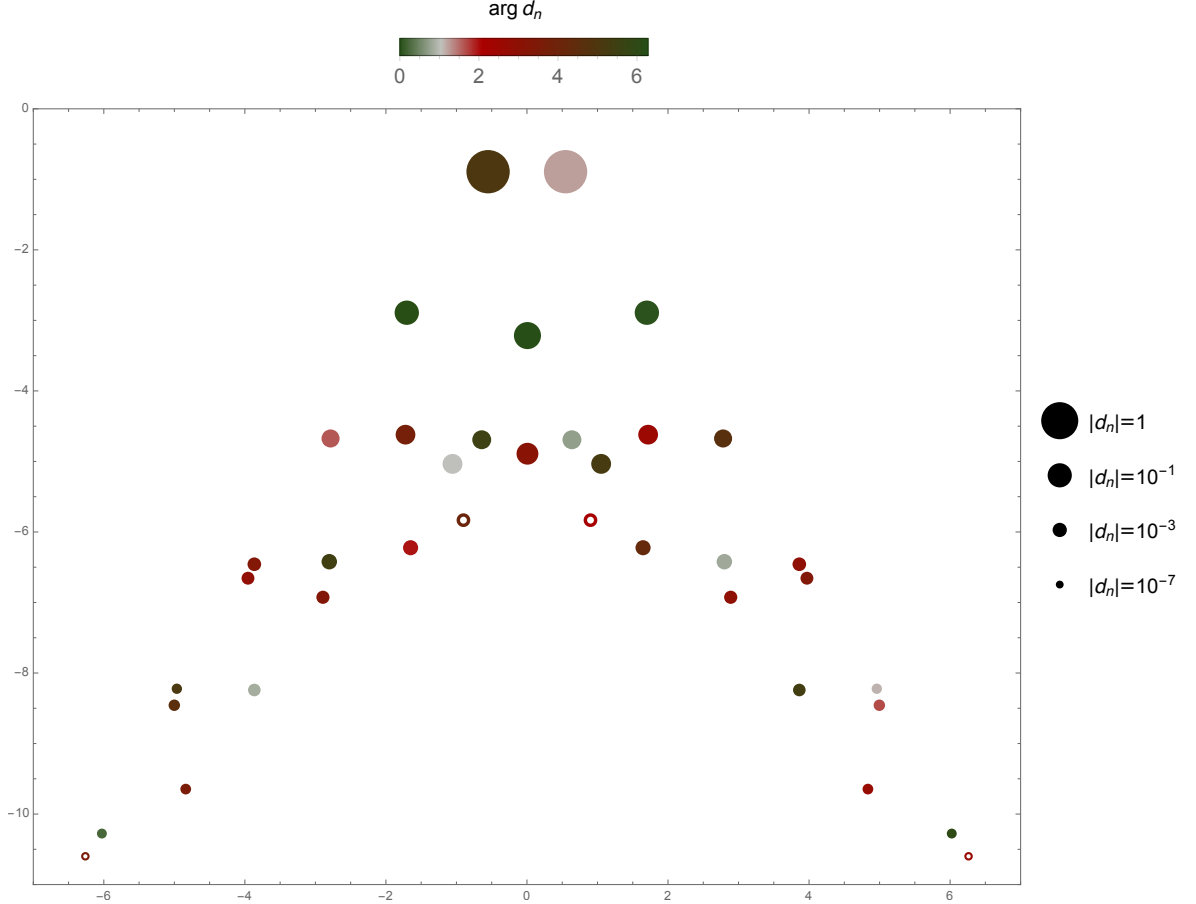
Figure 3: The spectrum of resonances in q = 4 SYK. The size and color of the dots indicate the magnitude and phase of d_n , which is given by the residue of G(\omega) at \omega_n as in (3.9). The solid dots have converged according to the criterion put forth in the main text, whereas the hollow dots have not yet converged.
